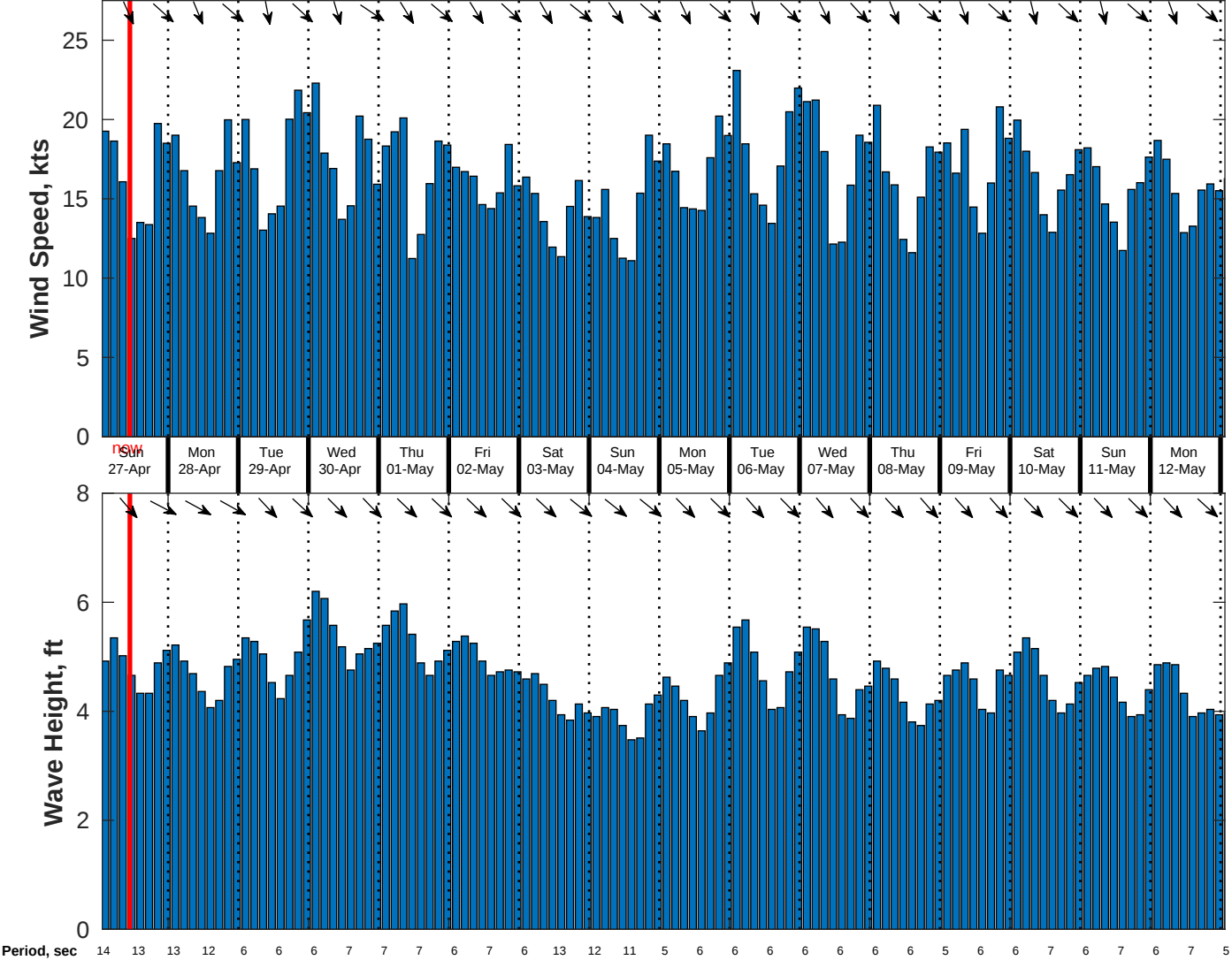
Wind & Wave Forecast for CSA (ONHYM) PPL EBS - Mauritania from 26-Apr-2025 01:00:00 to 12-May-2025 01:00:00
