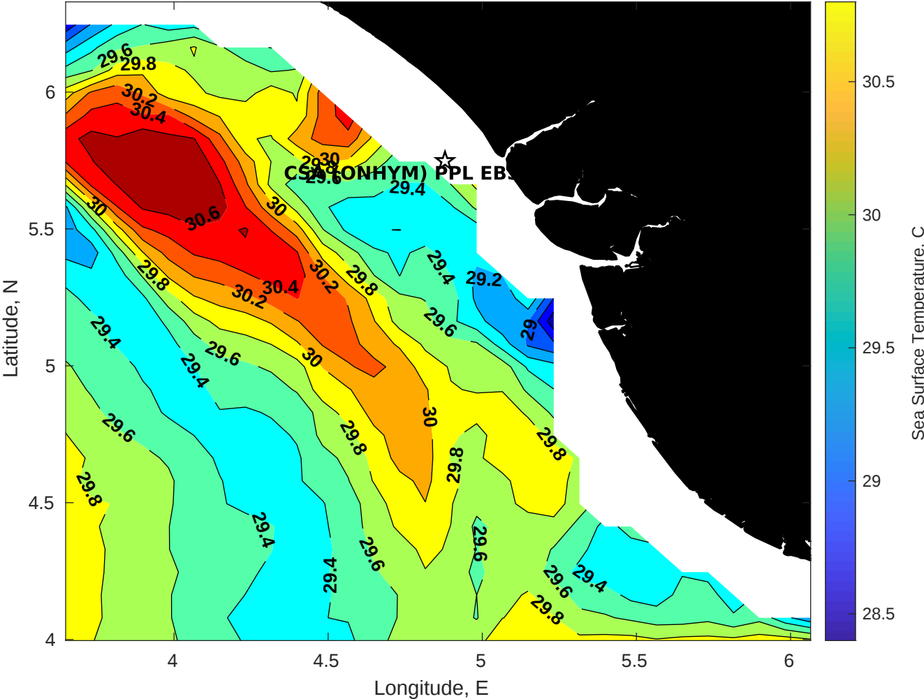
SST for CSA (ONHYM) PPL EBS - Nigeria at 25-Apr-2025 00:00:00
