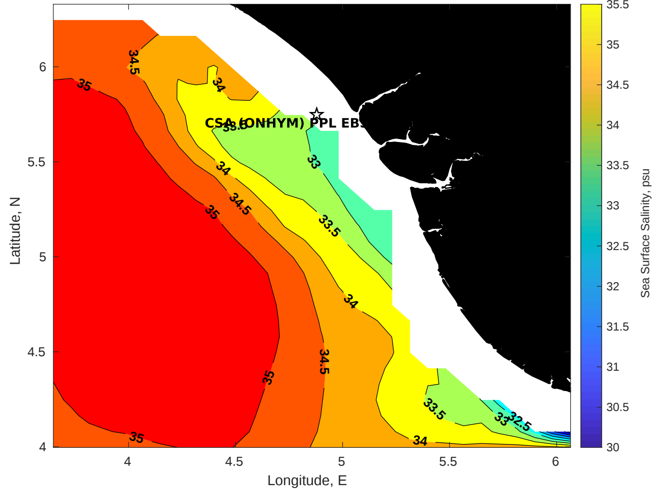
Surface Salinity for CSA (ONHYM) PPL EBS - Nigeria at 25-Apr-2025 00:00:00
