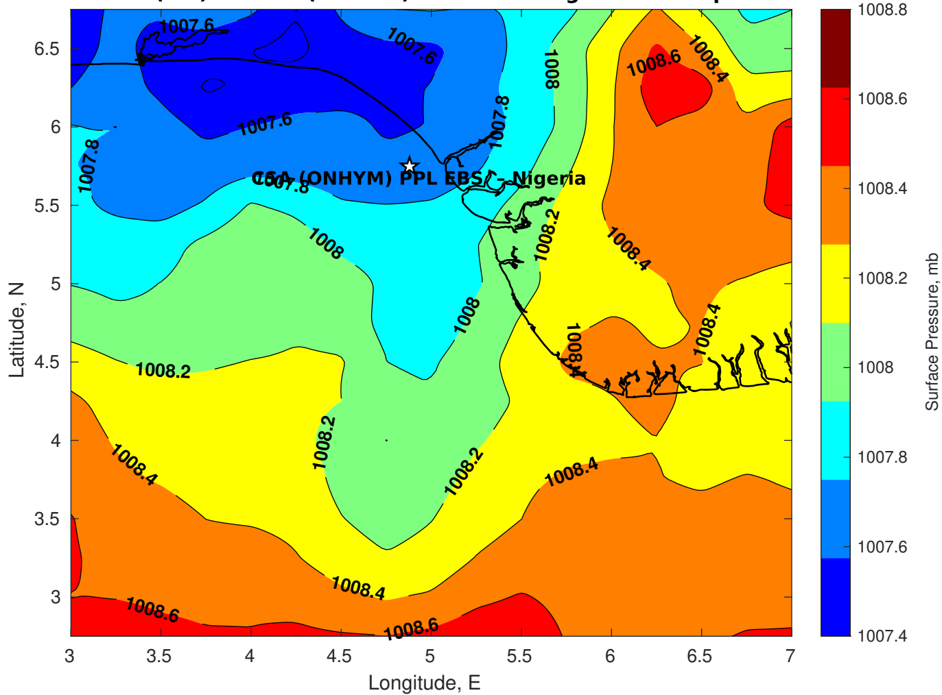
Surface Pressure (mb) for CSA (ONHYM) PPL EBS - Nigeria at 26-Apr-2025 00:00:00
