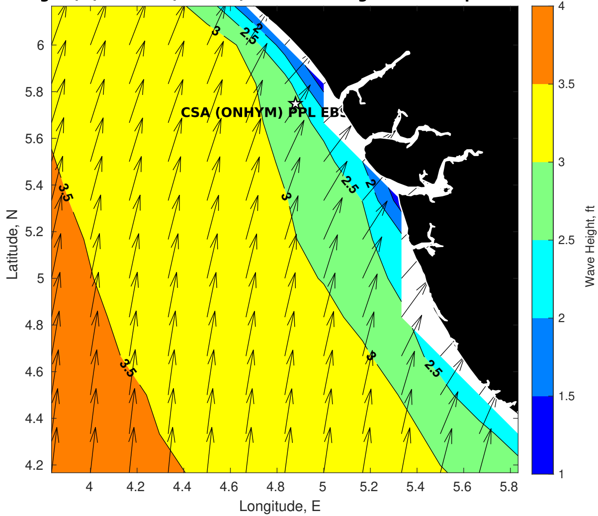
Wave Height (ft) for CSA (ONHYM) PPL EBS - Nigeria at 26-Apr-2025 09:00:00
