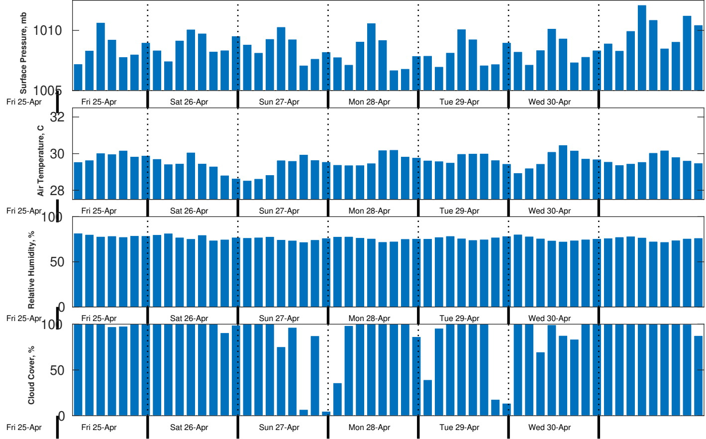
Met Forecast for CSA (ONHYM) PPL EBS - Nigeria from 26-Apr-2025 00:00:00 to 03-May-2025 00:00:00
