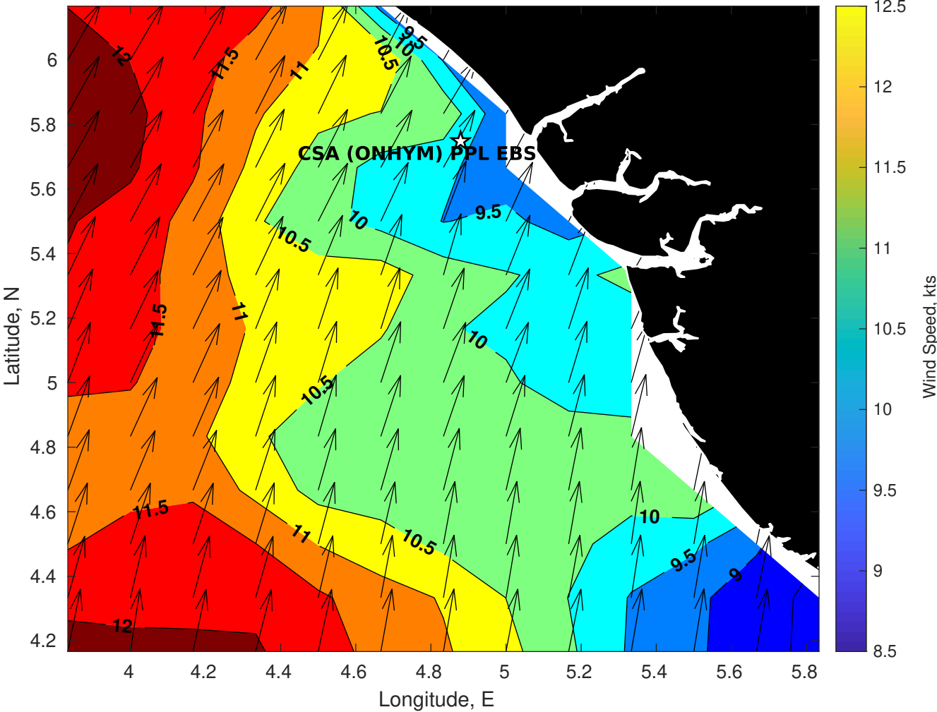
Winds (kts) for CSA (ONHYM) PPL EBS - Nigeria at 26-Apr-2025 09:00:00
