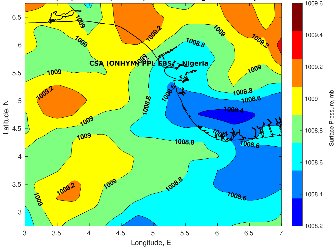
Surface Pressure (mb) for CSA (ONHYM) PPL EBS - Nigeria at 28-Apr-2025 00:00:00
