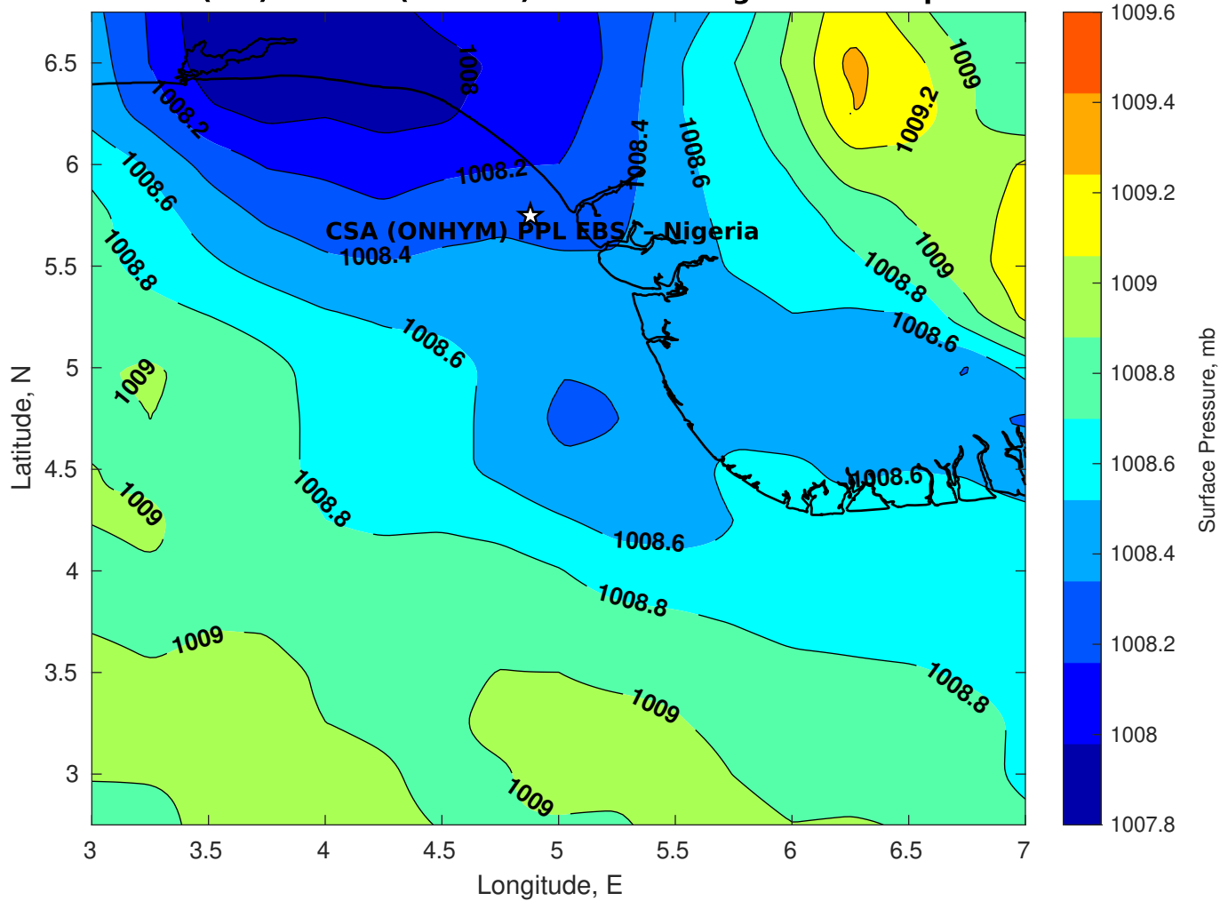
Surface Pressure (mb) for CSA (ONHYM) PPL EBS - Nigeria at 27-Apr-2025 00:00:00
