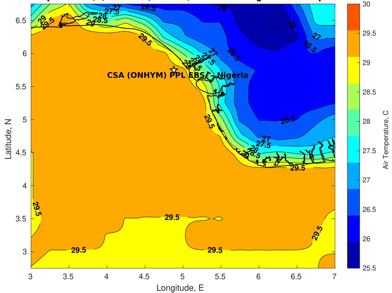
Air Temperature (C) for CSA (ONHYM) PPL EBS - Nigeria at 26-Apr-2025
