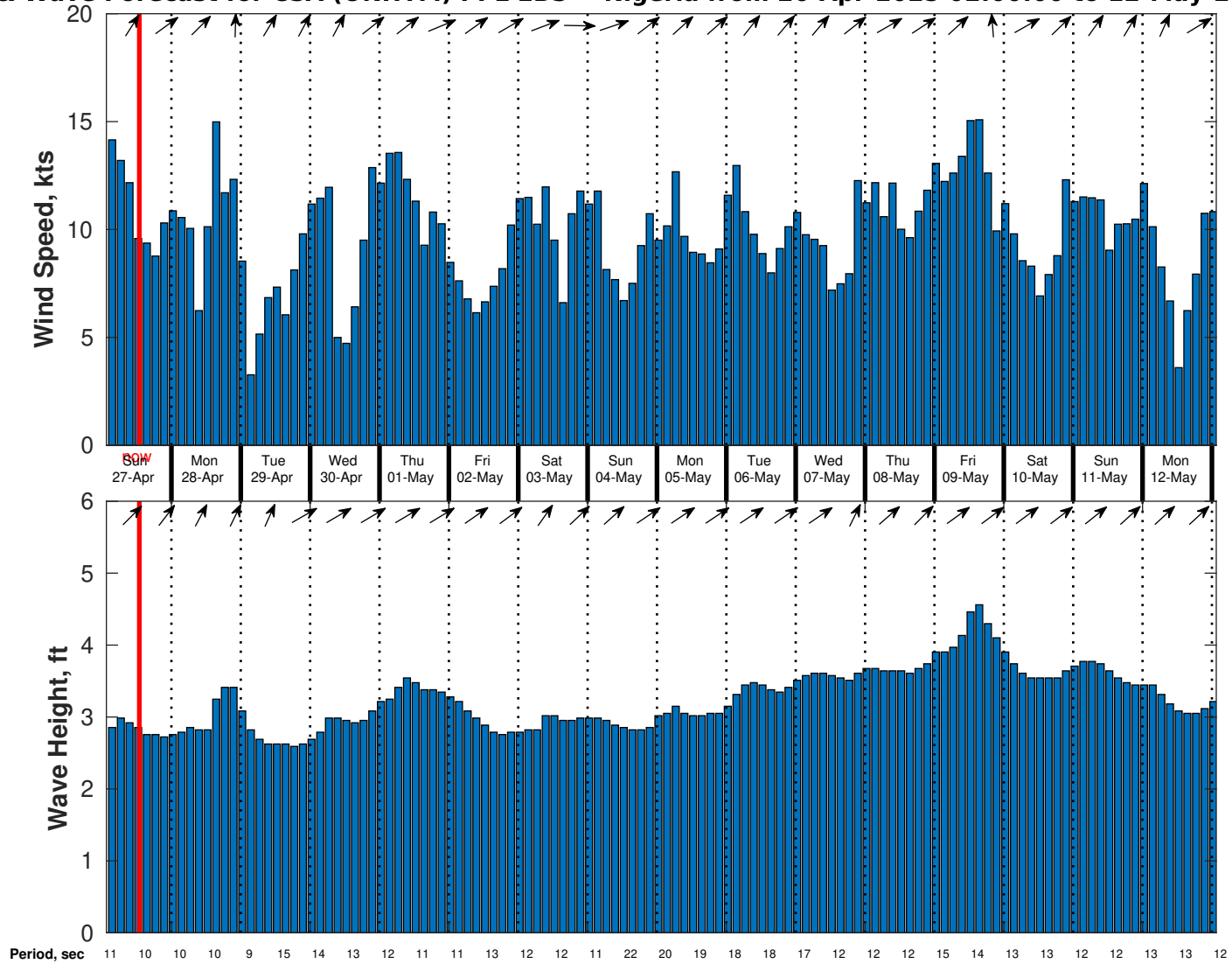
Wind & Wave Forecast for CSA (ONHYM) PPL EBS - Nigeria from 26-Apr-2025 02:00:00 to 12-May-2025 02:00:00
