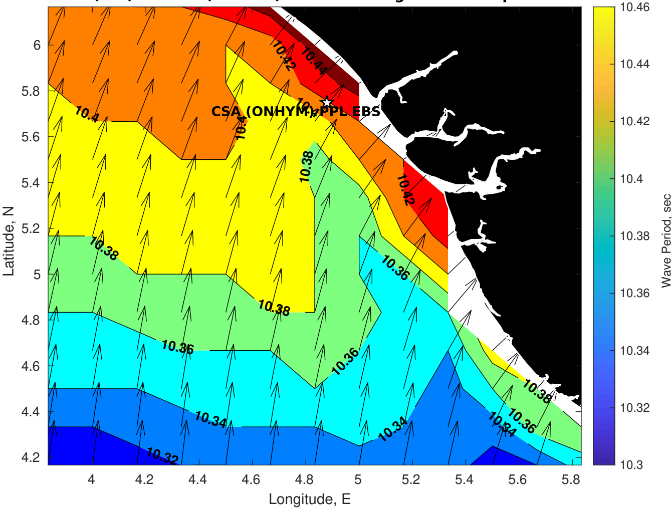
Wave Period (sec) for CSA (ONHYM) PPL EBS - Nigeria at 26-Apr-2025 09:00:00
