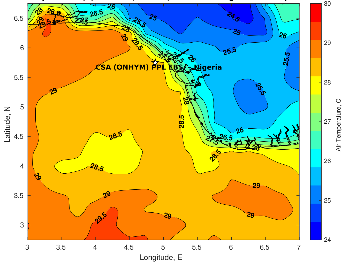
Air Temperature (C) for CSA (ONHYM) PPL EBS - Nigeria at 26-Apr-2025
