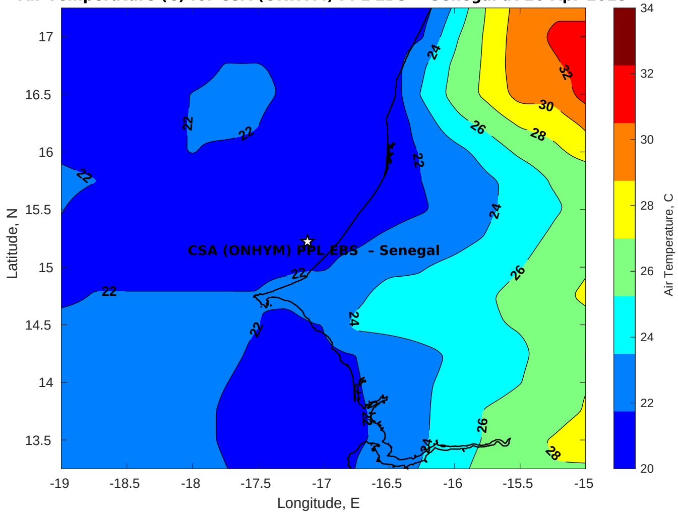
Air Temperature (C) for CSA (ONHYM) PPL EBS - Senegal at 26-Apr-2025
