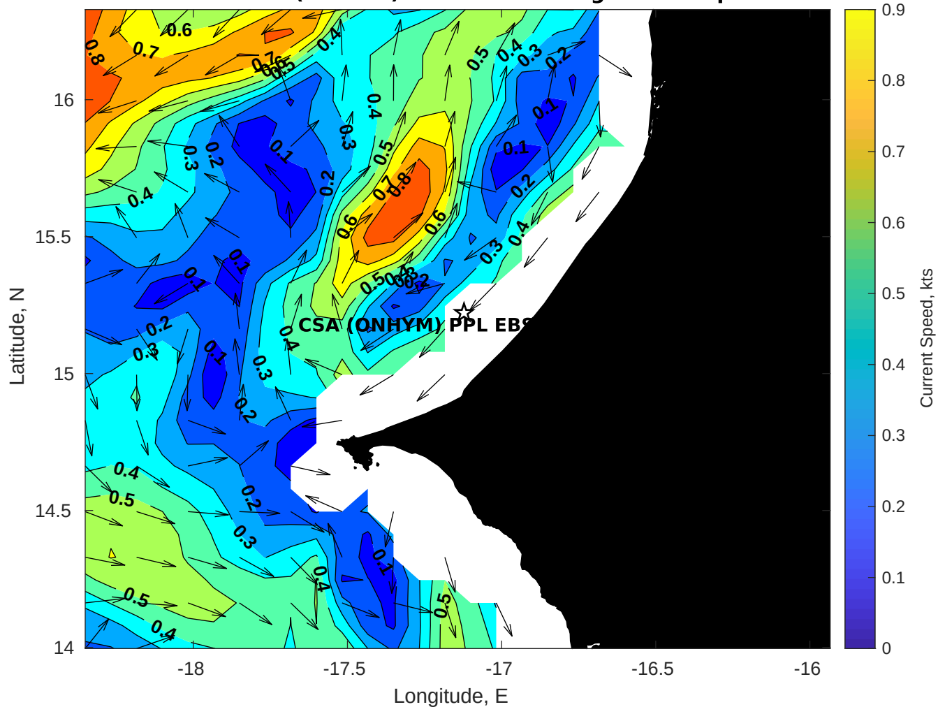
Surface Currents for CSA (ONHYM) PPL EBS - Senegal at 25-Apr-2025 00:00:00
