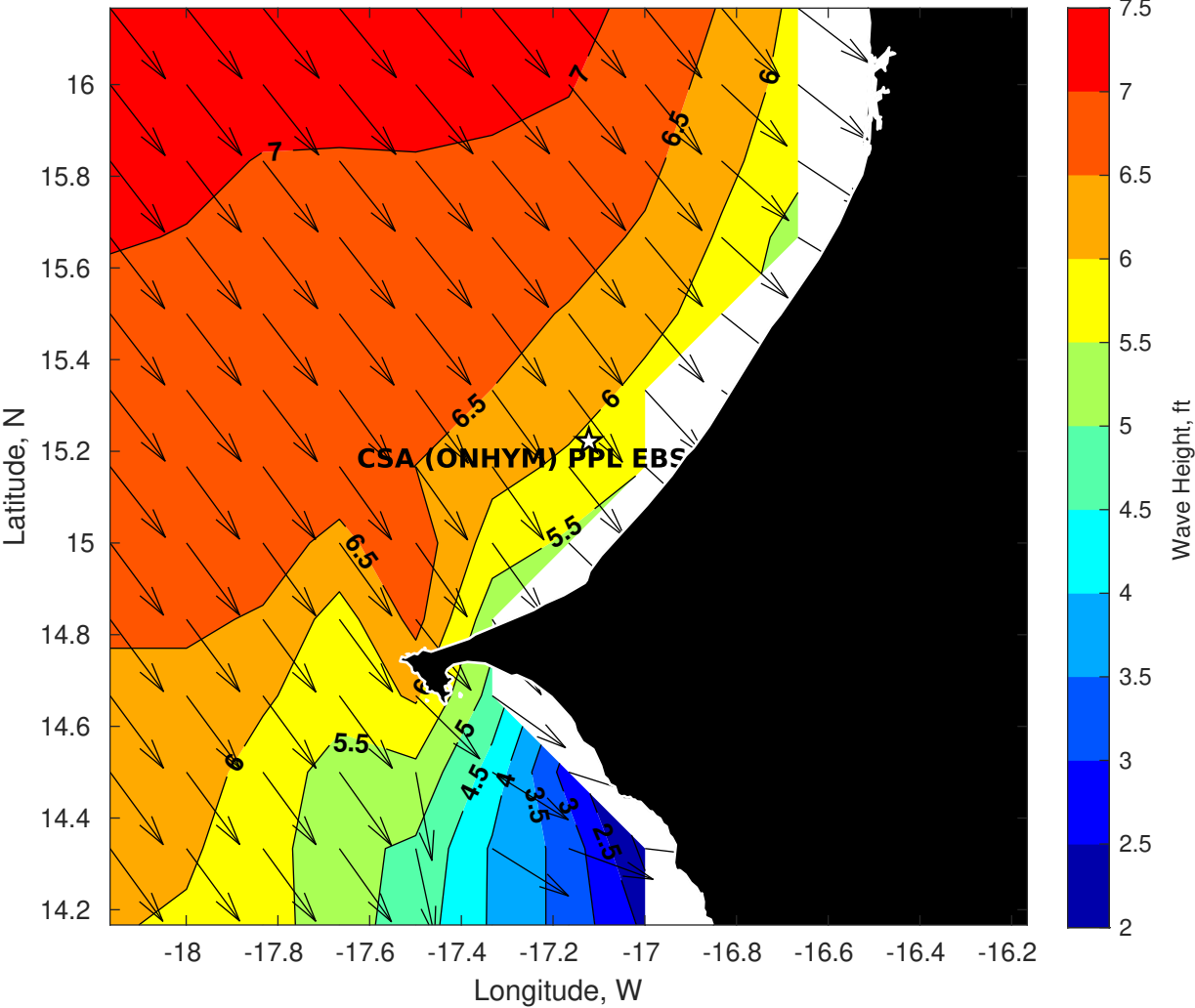
Wave Height (ft) for CSA (ONHYM) PPL EBS - Senegal at 26-Apr-2025 09:00:00
