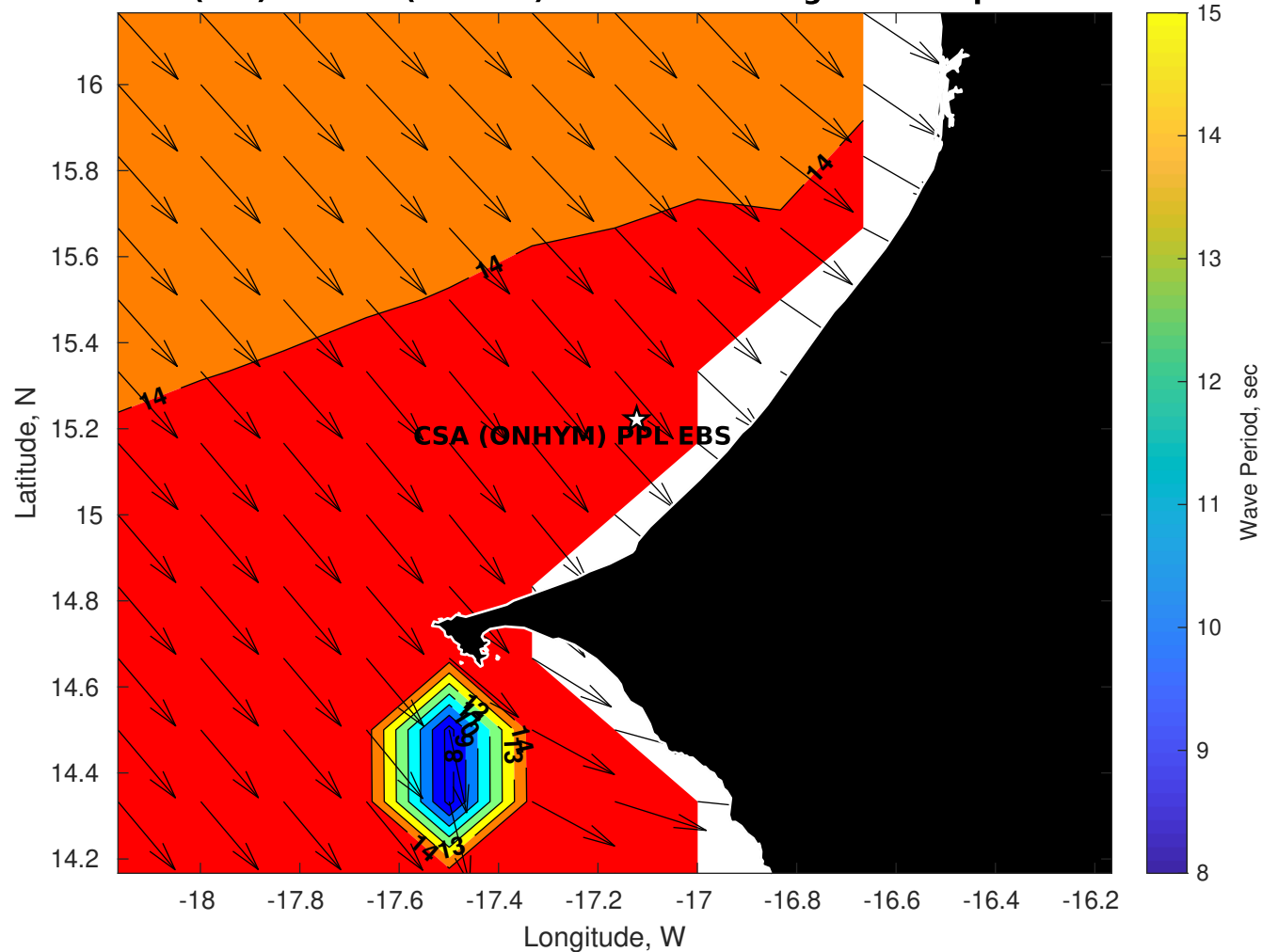
Wave Period (sec) for CSA (ONHYM) PPL EBS - Senegal at 26-Apr-2025 09:00:00
