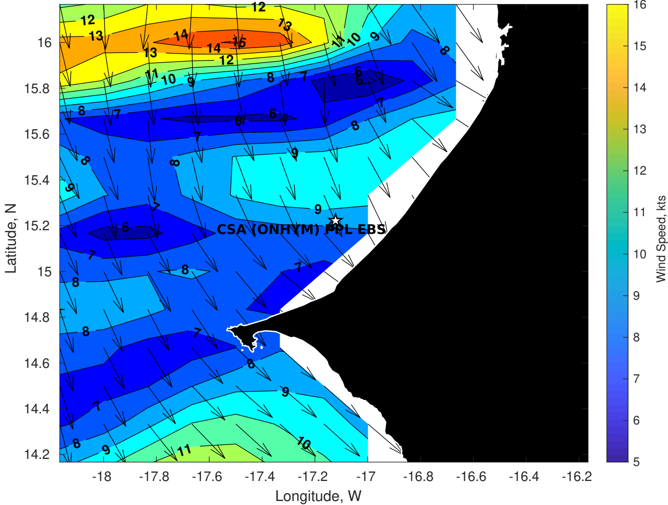
Winds (kts) for CSA (ONHYM) PPL EBS - Senegal at 26-Apr-2025 09:00:00
