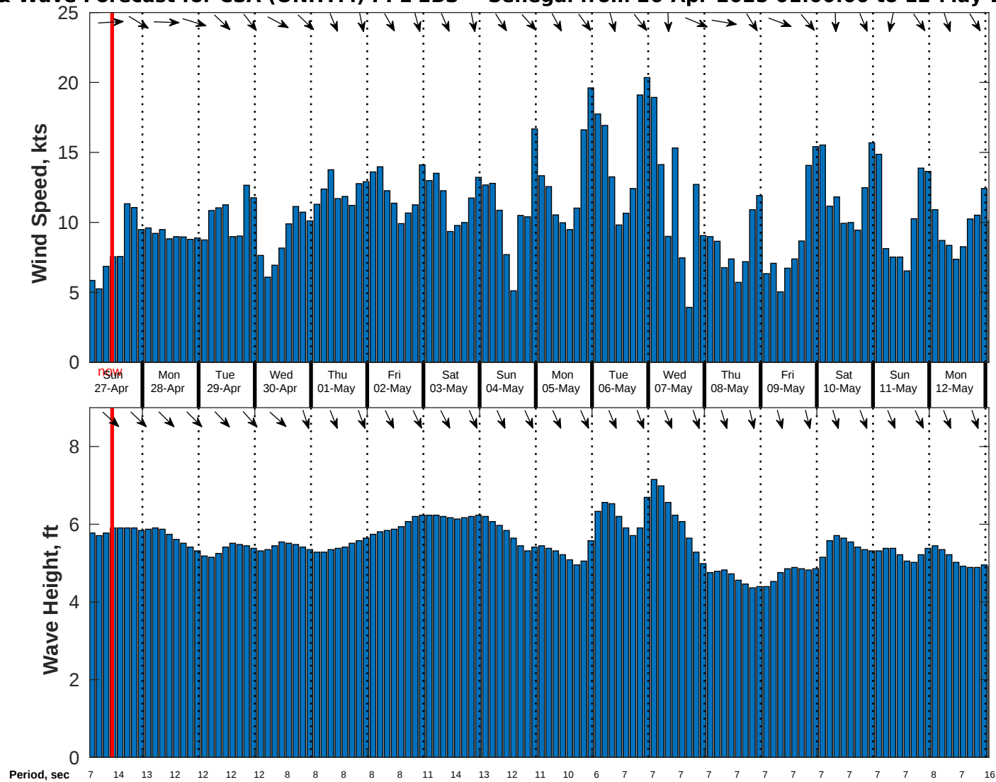
Wind & Wave Forecast for CSA (ONHYM) PPL EBS - Senegal from 26-Apr-2025 01:00:00 to 12-May-2025 01:00:00
