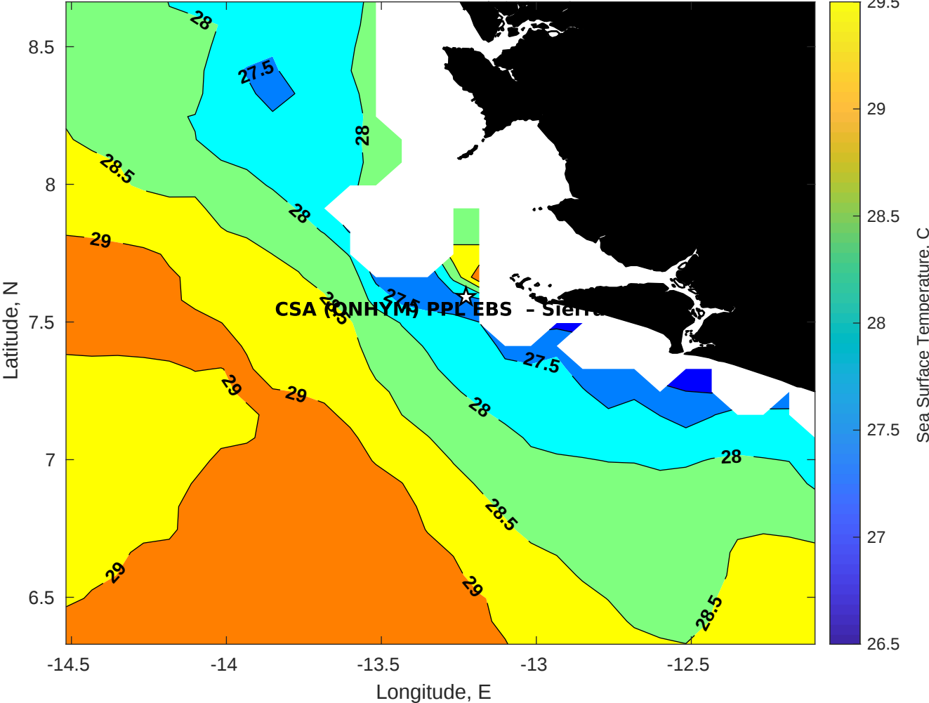
SST for CSA (ONHYM) PPL EBS - Sierra Leone at 25-Apr-2025 00:00:00
