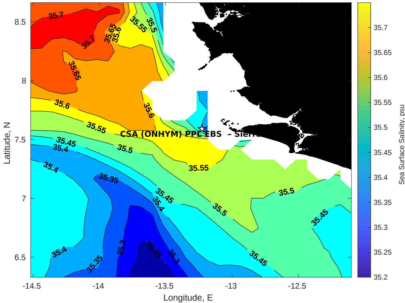
Surface Salinity for CSA (ONHYM) PPL EBS - Sierra Leone at 25-Apr-2025 00:00:00
