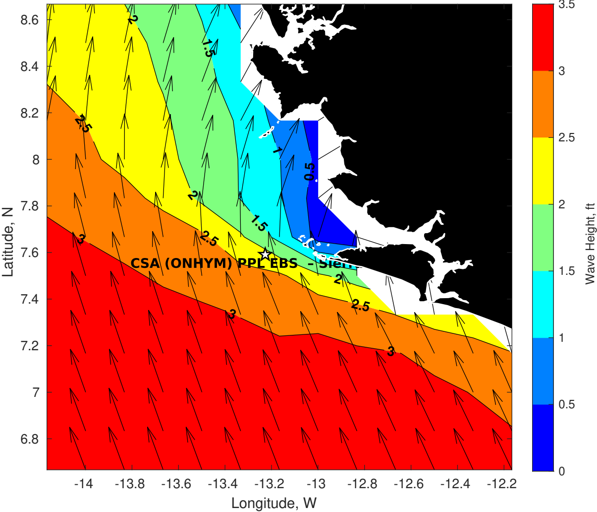
Wave Height (ft) for CSA (ONHYM) PPL EBS - Sierra Leone at 26-Apr-2025 09:00:00
