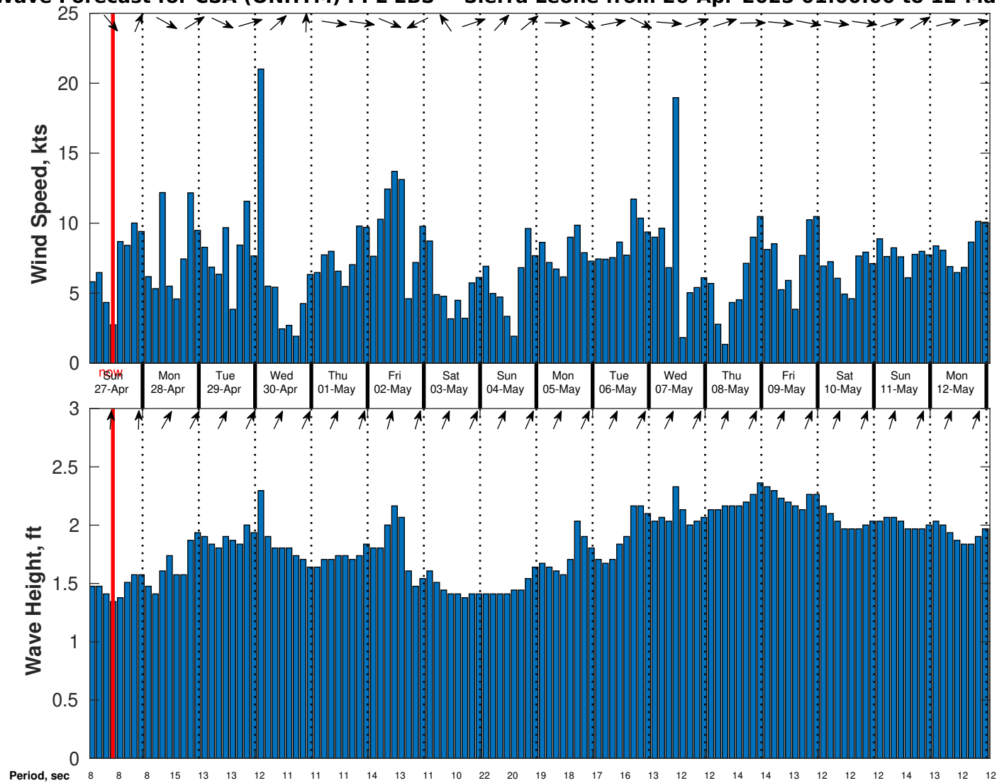
Wind & Wave Forecast for CSA (ONHYM) PPL EBS - Sierra Leone from 26-Apr-2025 01:00:00 to 12-May-2025 01:00:00
