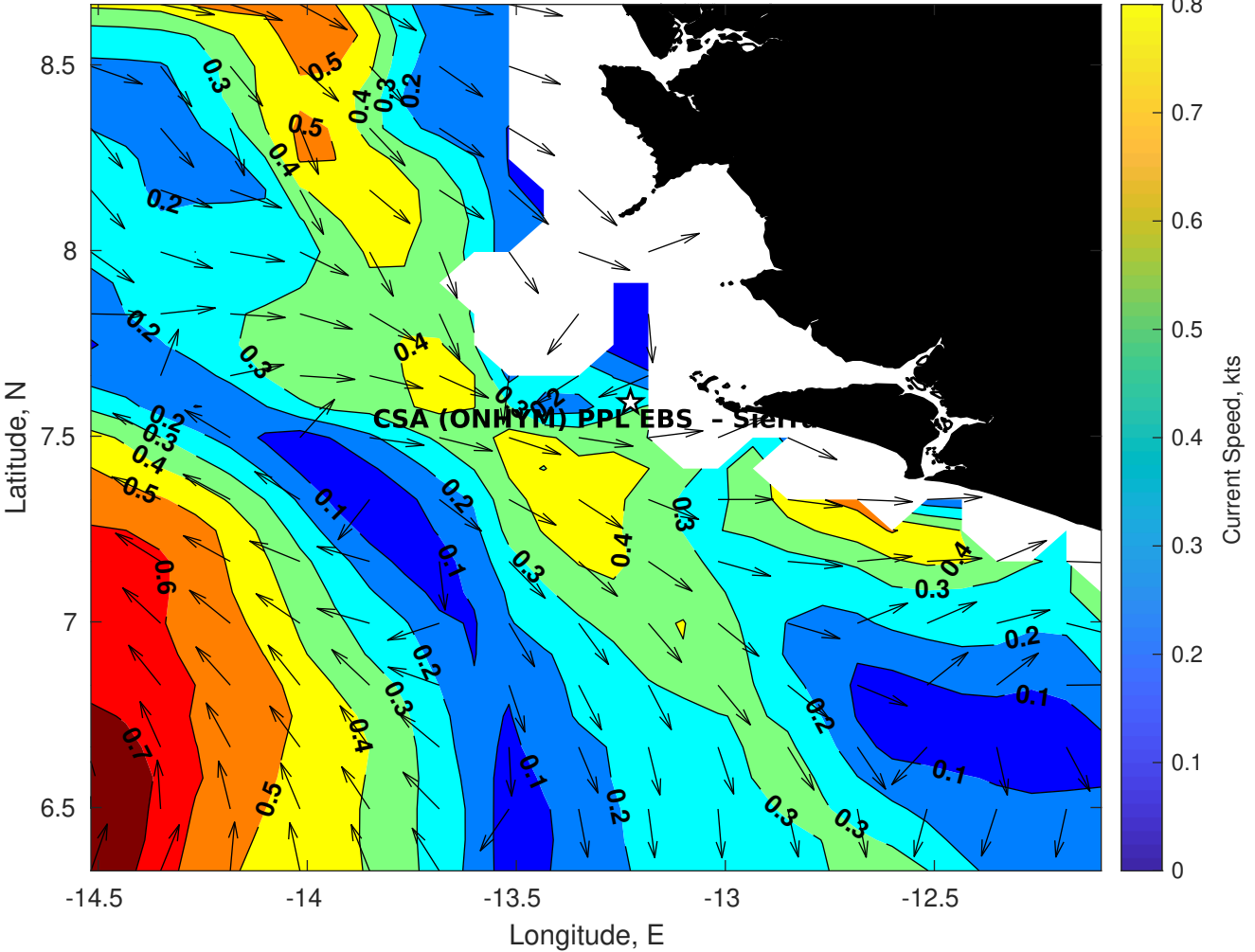
Surface Currents for CSA (ONHYM) PPL EBS - Sierra Leone at 25-Apr-2025 00:00:00
