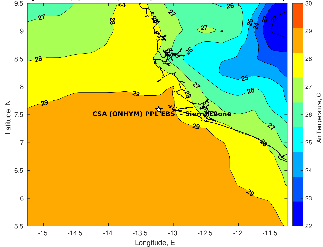
Air Temperature (C) for CSA (ONHYM) PPL EBS - Sierra Leone at 26-Apr-2025
