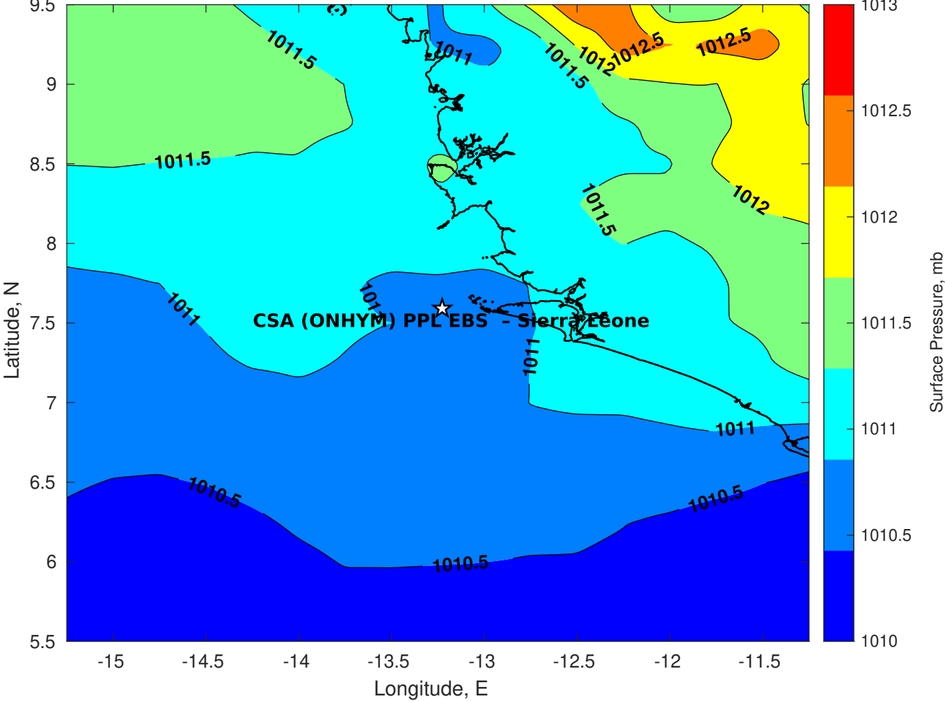
Surface Pressure (mb) for CSA (ONHYM) PPL EBS - Sierra Leone at 27-Apr-2025 00:00:00
