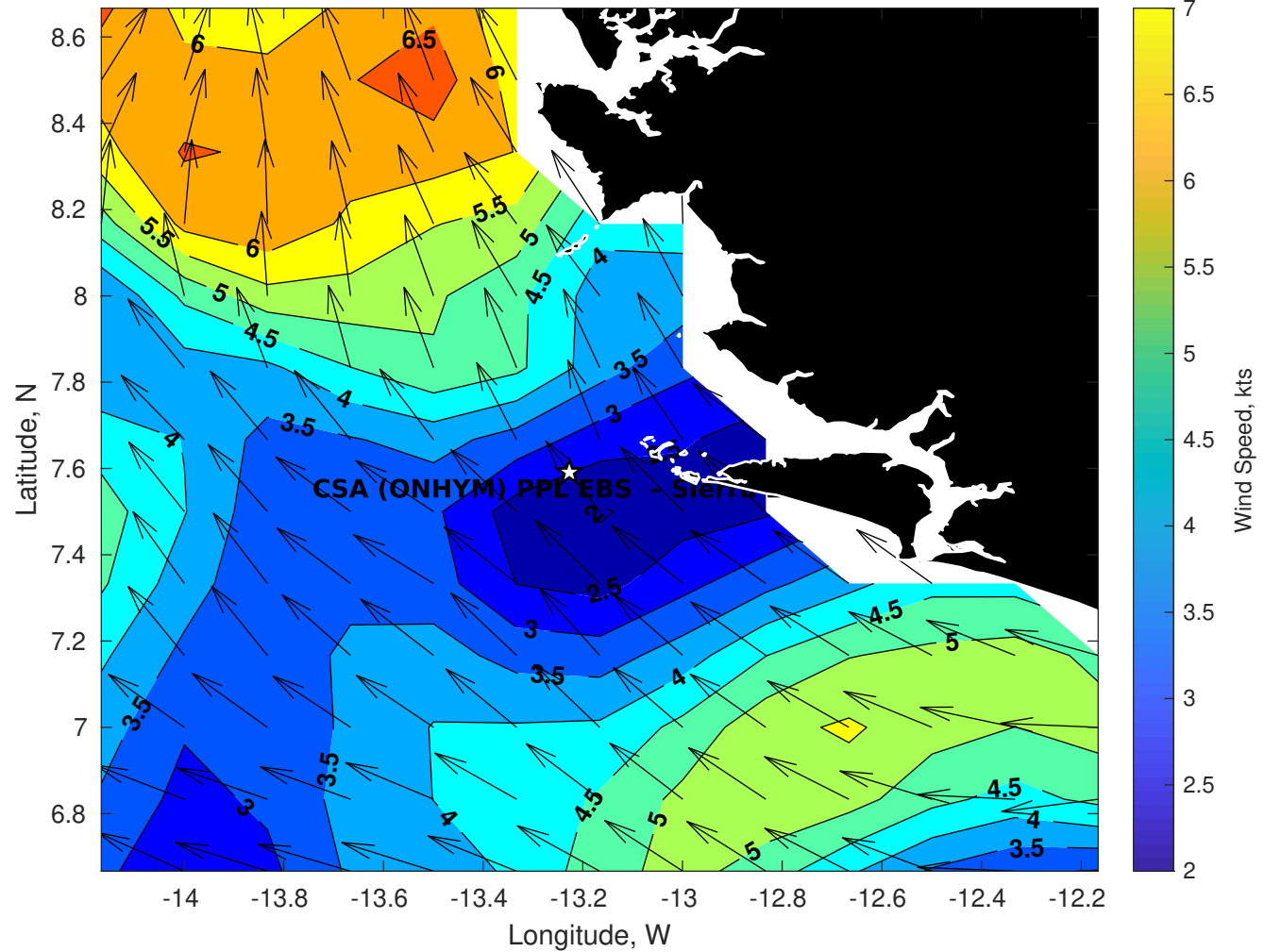
Winds (kts) for CSA (ONHYM) PPL EBS - Sierra Leone at 26-Apr-2025 09:00:00
