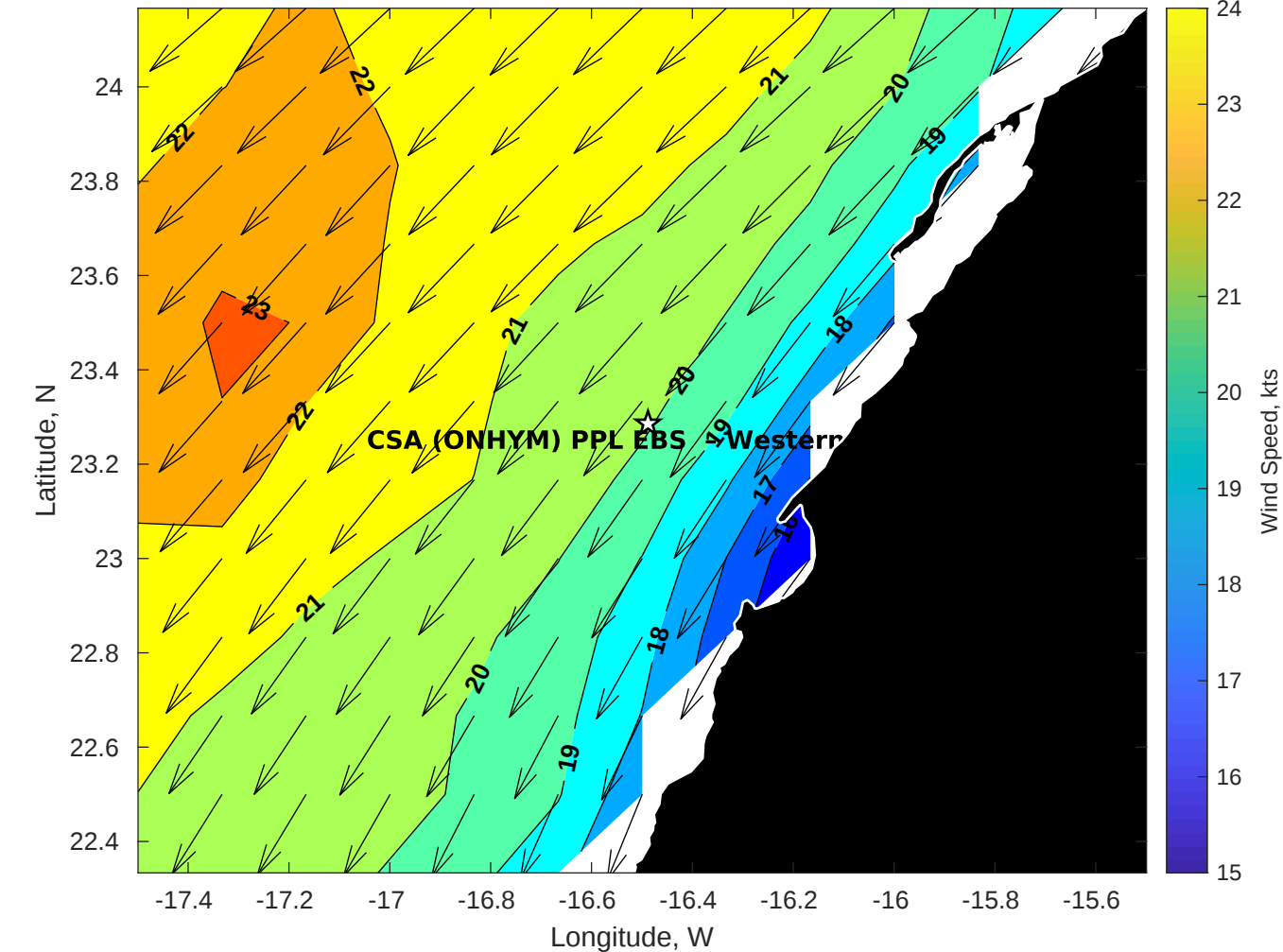
Winds (kts) for CSA (ONHYM) PPL EBS - Western Sahara at 26-Apr-2025 09:00:00
