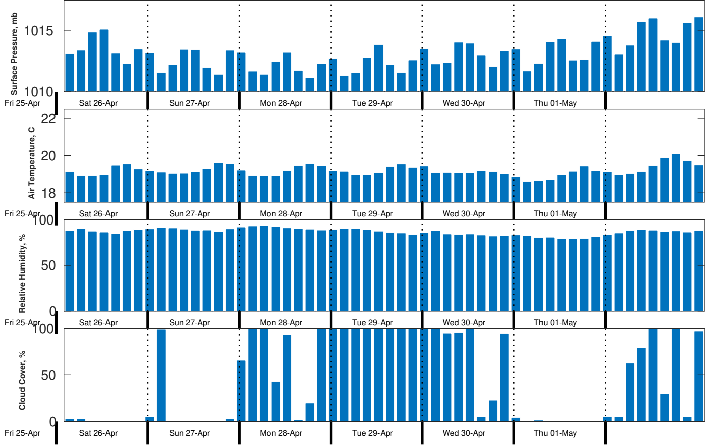
Met Forecast for CSA (ONHYM) PPL EBS - Western Sahara from 26-Apr-2025 00:00:00 to 03-May-2025 00:00:00
