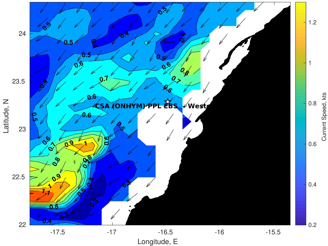
Surface Currents for CSA (ONHYM) PPL EBS - Western Sahara at 25-Apr-2025 00:00:00
