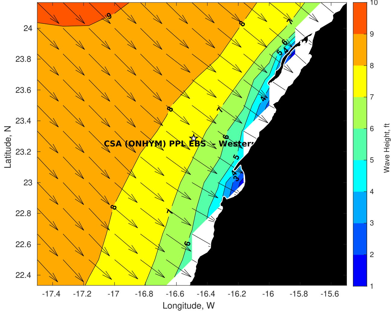
Wave Height (ft) for CSA (ONHYM) PPL EBS - Western Sahara at 26-Apr-2025 09:00:00
