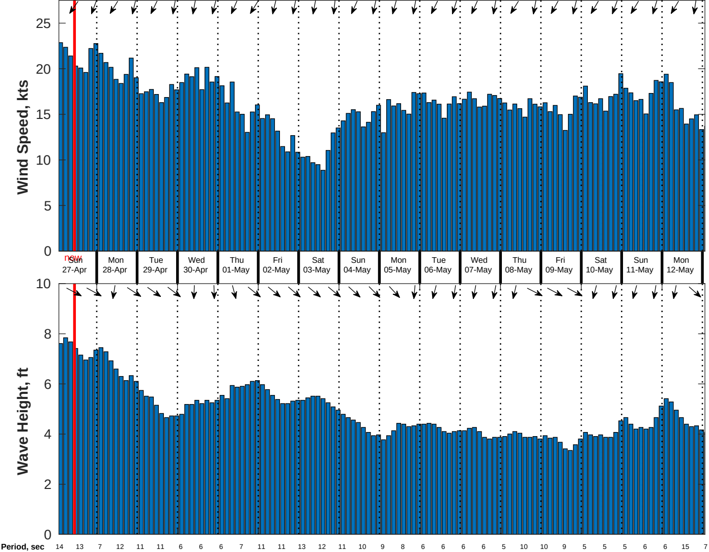
Wind & Wave Forecast for CSA (ONHYM) PPL EBS - Western Sahara from 26-Apr-2025 01:00:00 to 12-May-2025 01:00:00
