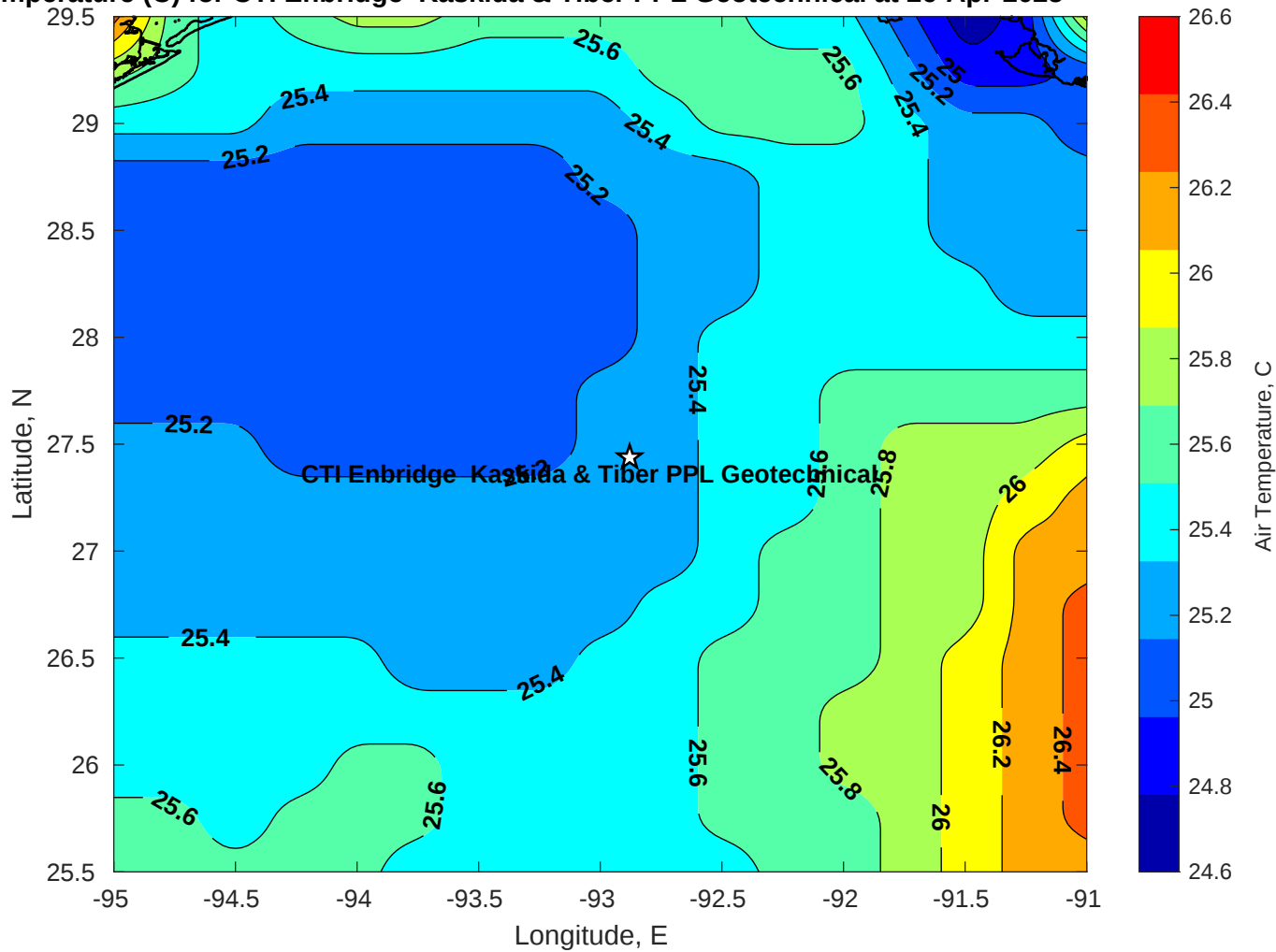
Air Temperature (C) for CTI Enbridge Kaskida & Tiber PPL Geotechnical at 26-Apr-2025
