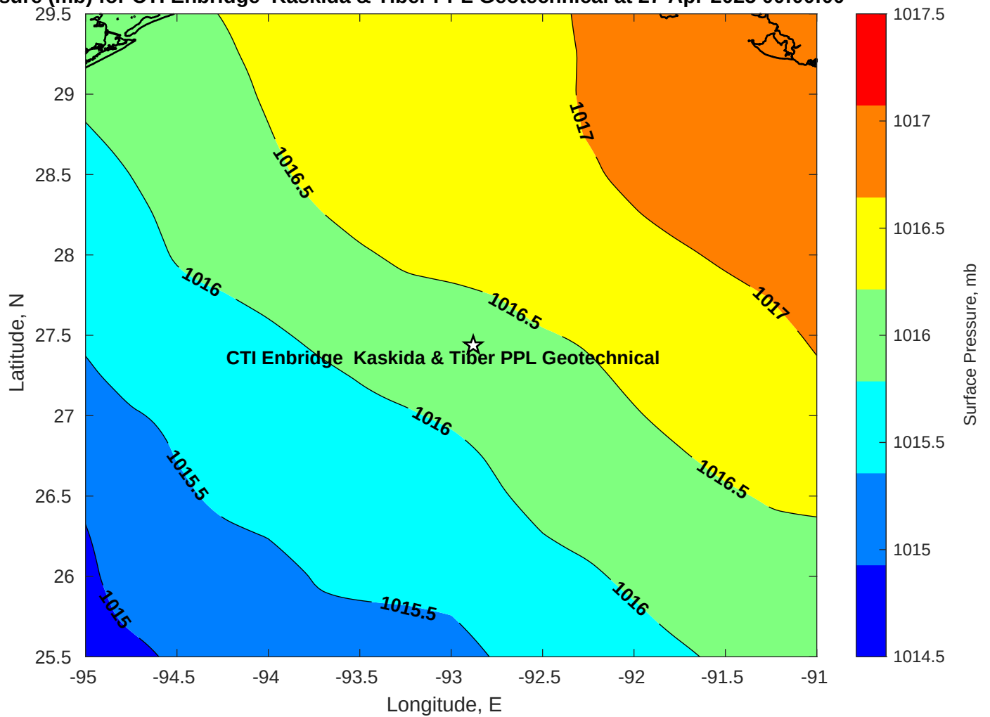
Surface Pressure (mb) for CTI Enbridge Kaskida & Tiber PPL Geotechnical at 27-Apr-2025 00:00:00
