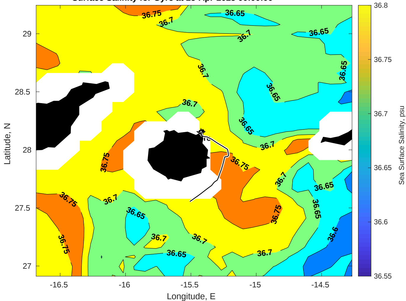
Surface Salinity for Gyre at 25-Apr-2025 00:00:00
