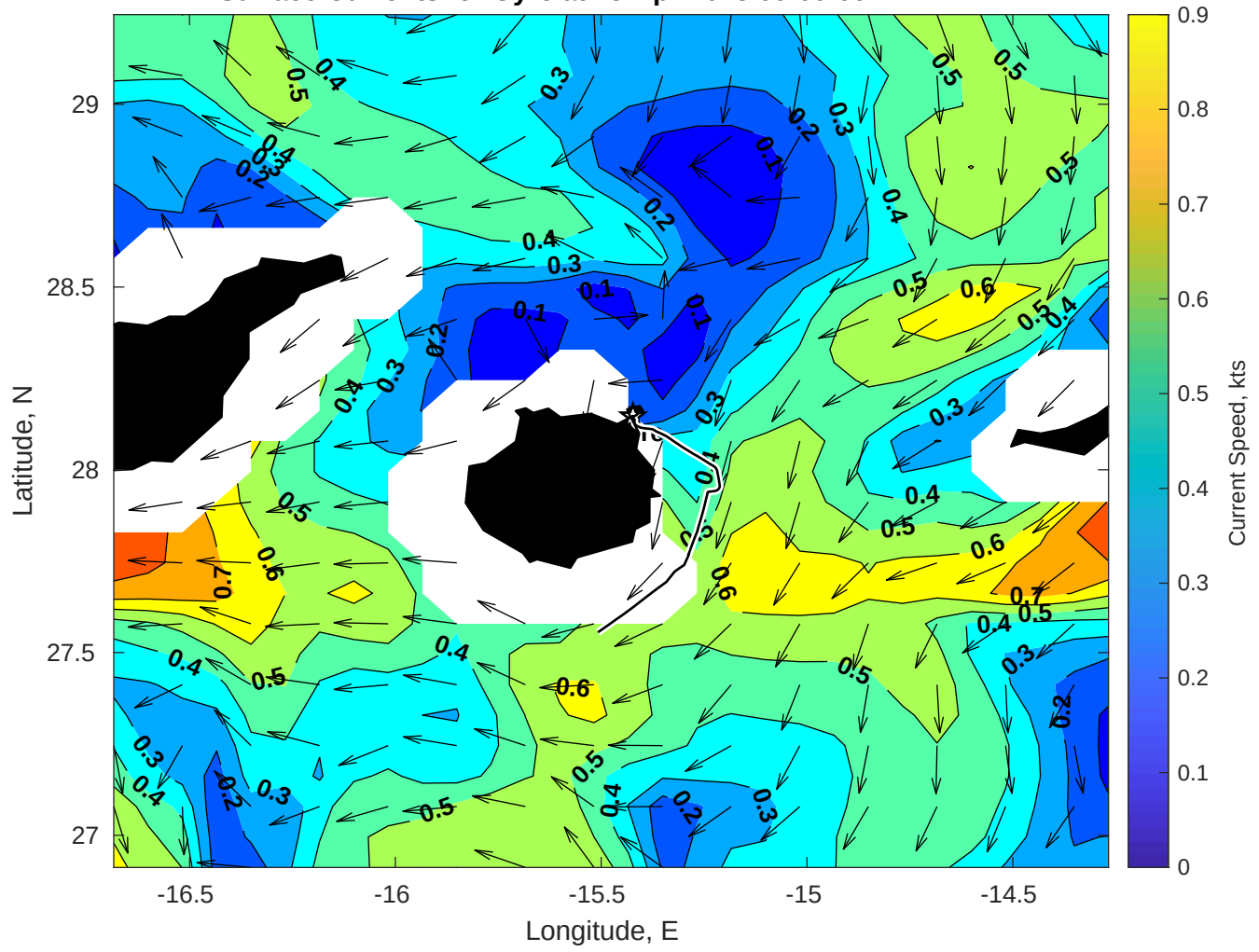
Surface Currents for Gyre at 25-Apr-2025 00:00:00
