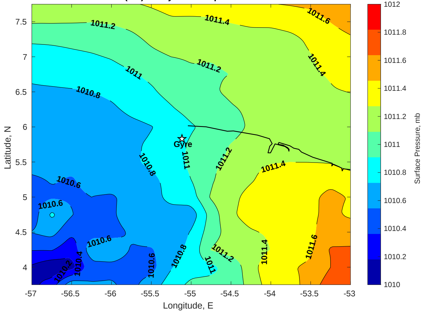
Surface Pressure (mb) for Gyre at 27-Apr-2025 00:00:00
