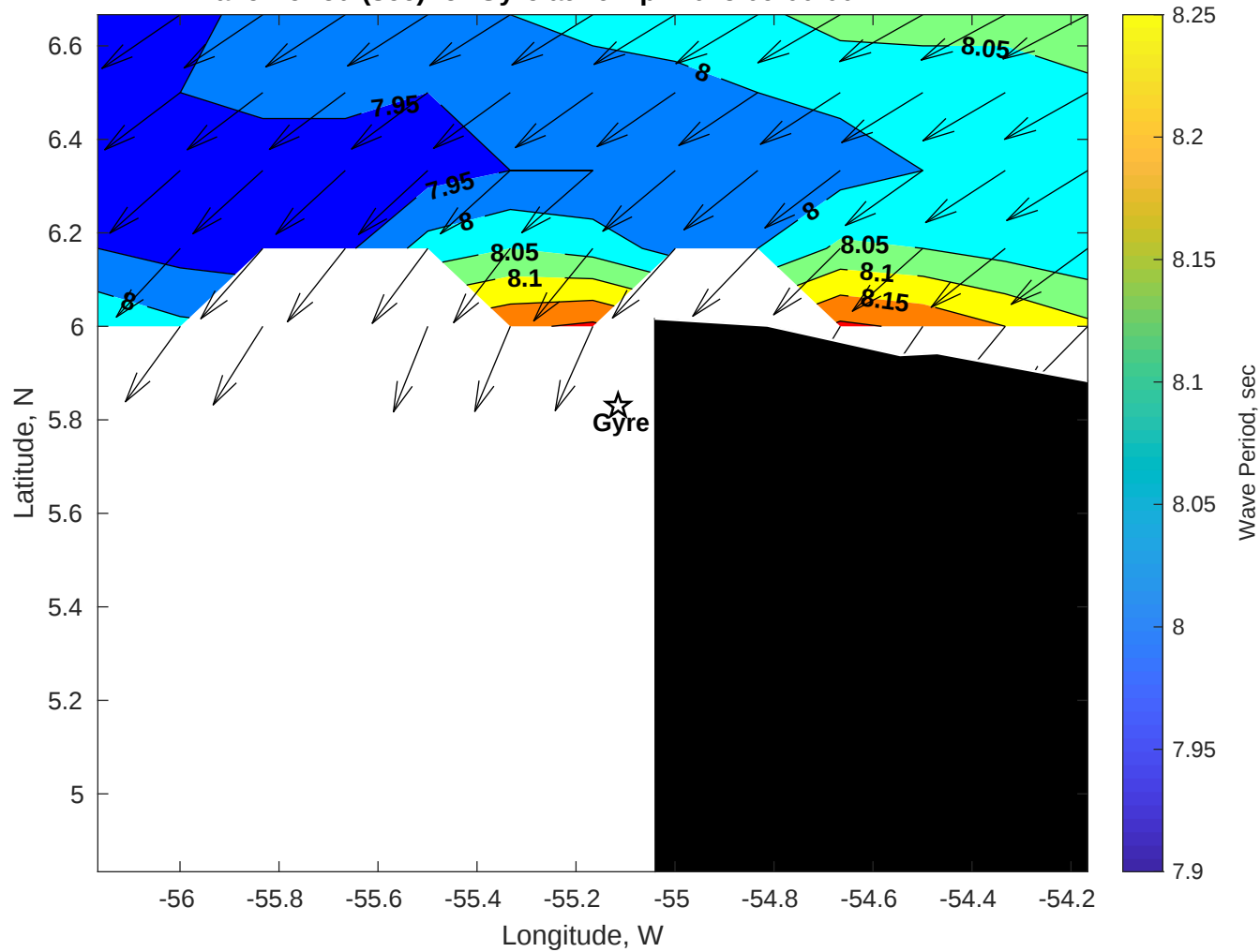
Wave Period (sec) for Gyre at 26-Apr-2025 09:00:00
