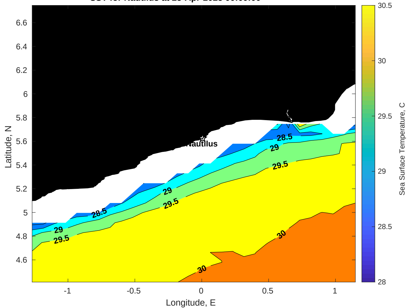
SST for Nautilus at 25-Apr-2025 00:00:00
