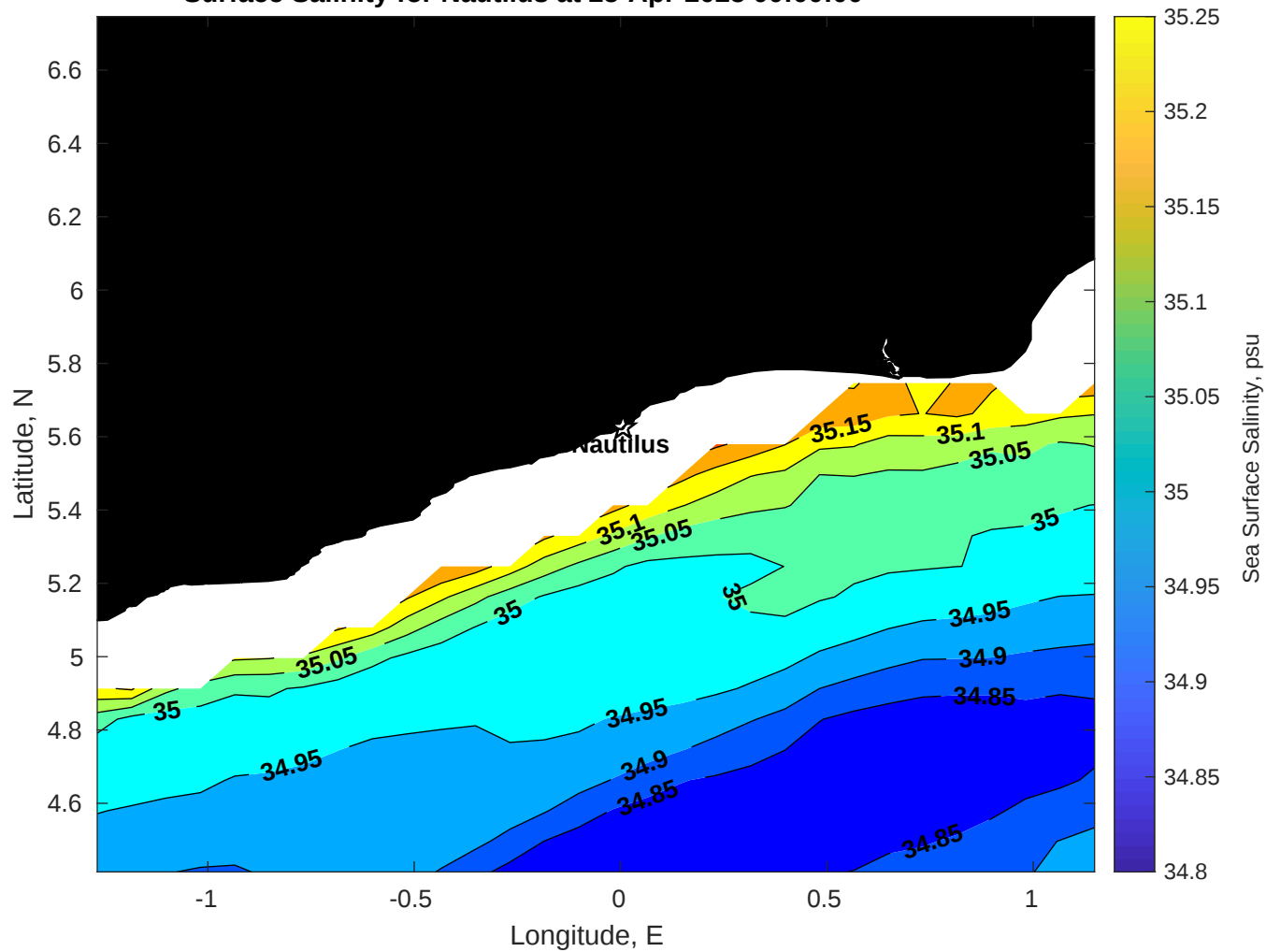
Surface Salinity for Nautilus at 25-Apr-2025 00:00:00
