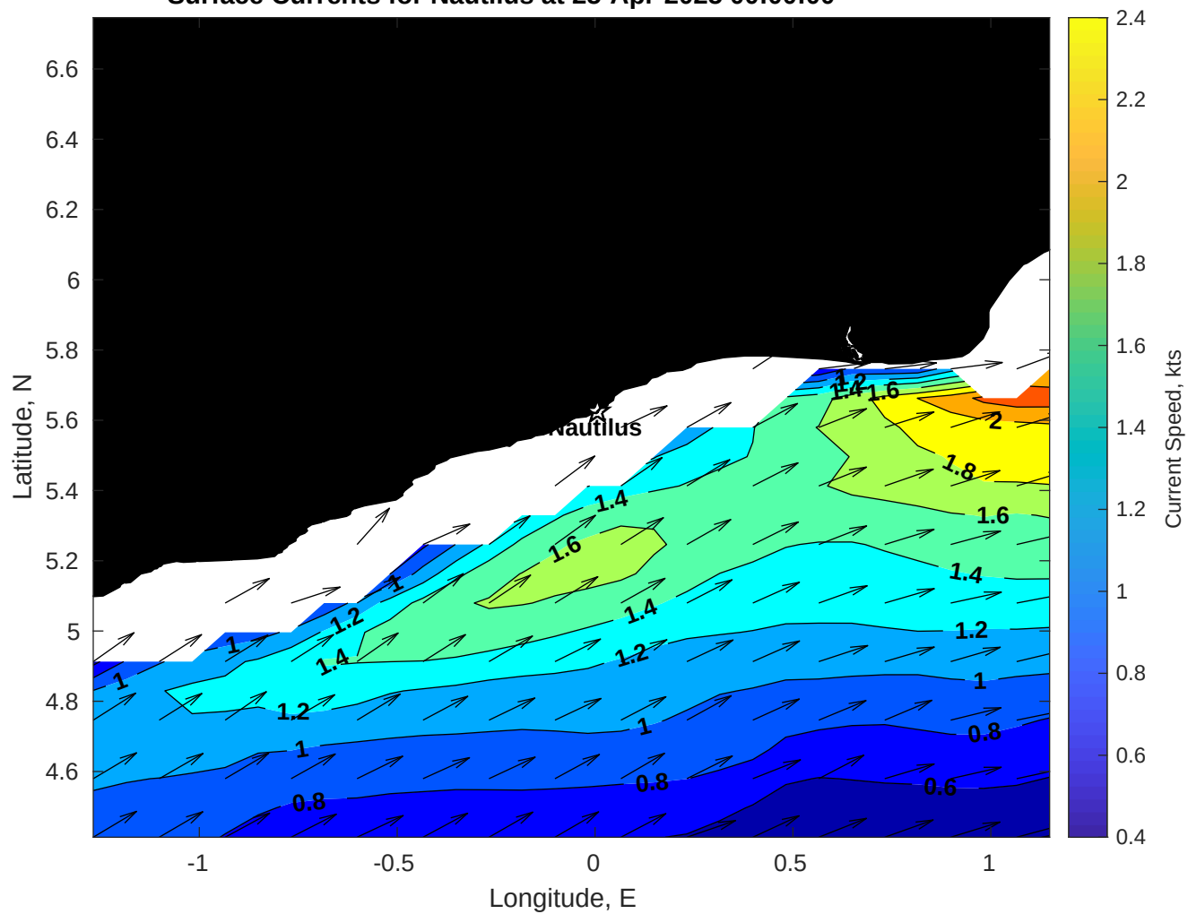
Surface Currents for Nautilus at 25-Apr-2025 00:00:00
