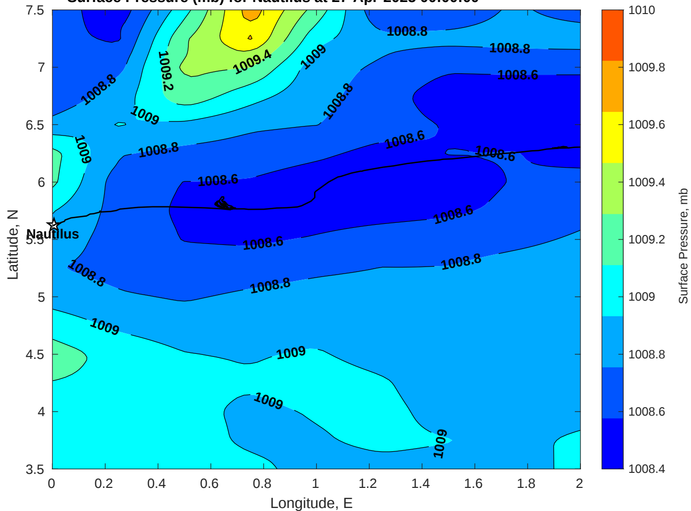
Surface Pressure (mb) for Nautilus at 27-Apr-2025 00:00:00
