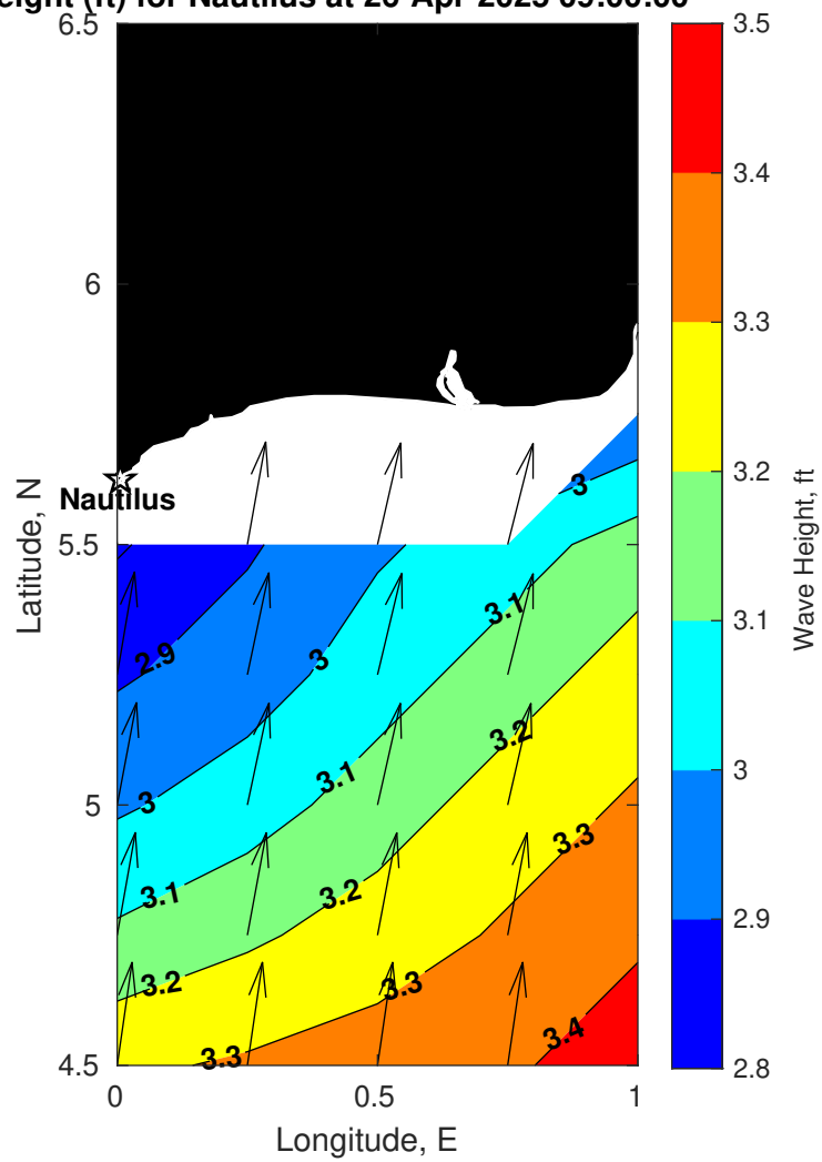
Wave Height (ft) for Nautilus at 26-Apr-2025 09:00:00
