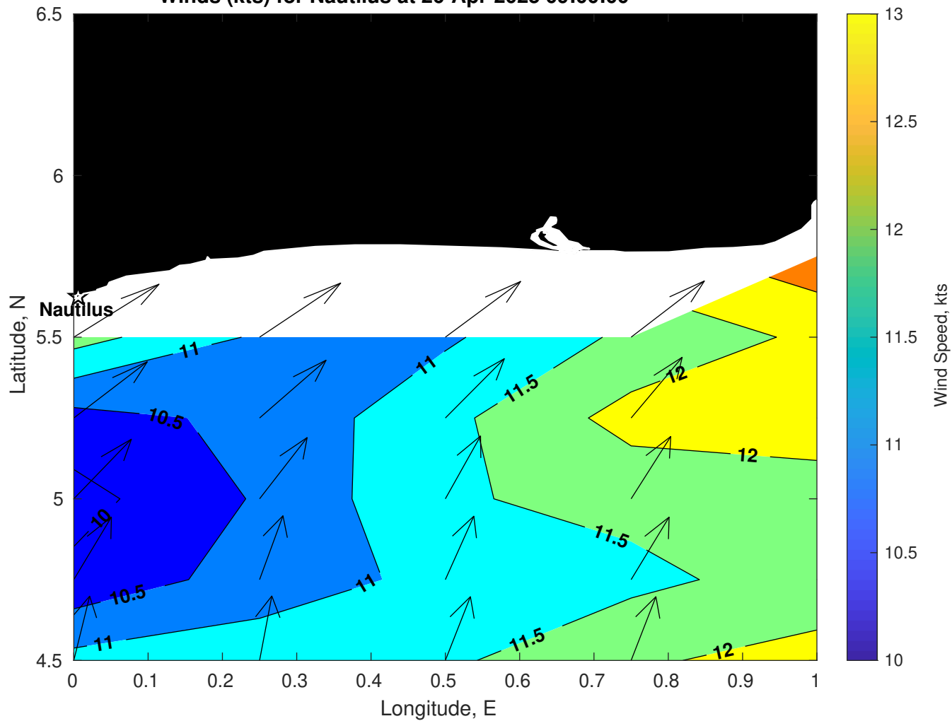
Winds (kts) for Nautilus at 26-Apr-2025 09:00:00
