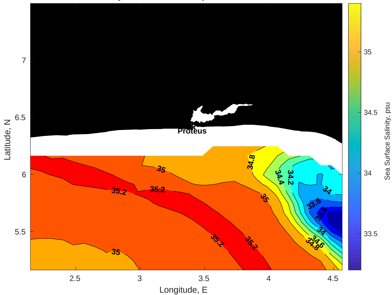
Surface Salinity for Proteus at 25-Apr-2025 00:00:00
