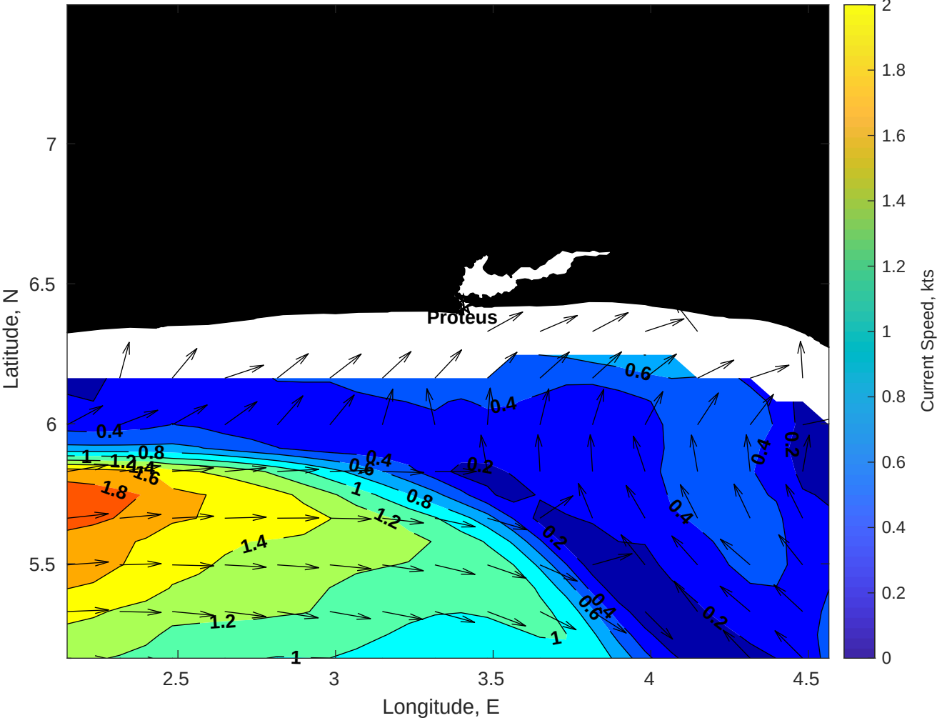
Surface Currents for Proteus at 25-Apr-2025 00:00:00
