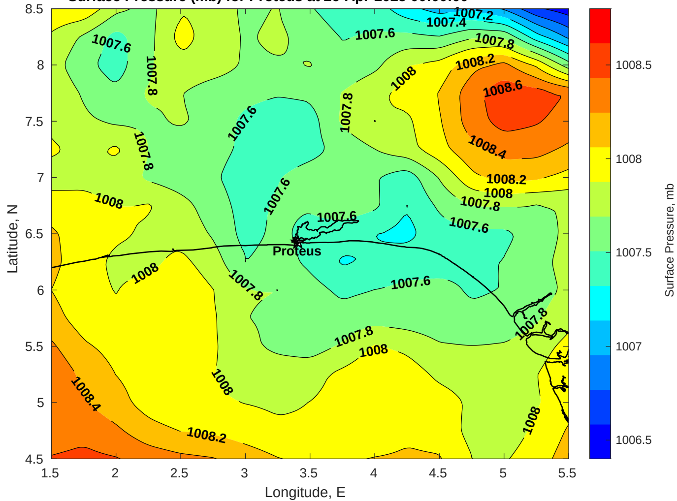
Surface Pressure (mb) for Proteus at 26-Apr-2025 00:00:00
