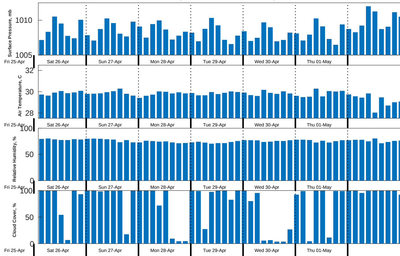
Met Forecast for Proteus from 26-Apr-2025 00:00:00 to 03-May-2025 00:00:00
