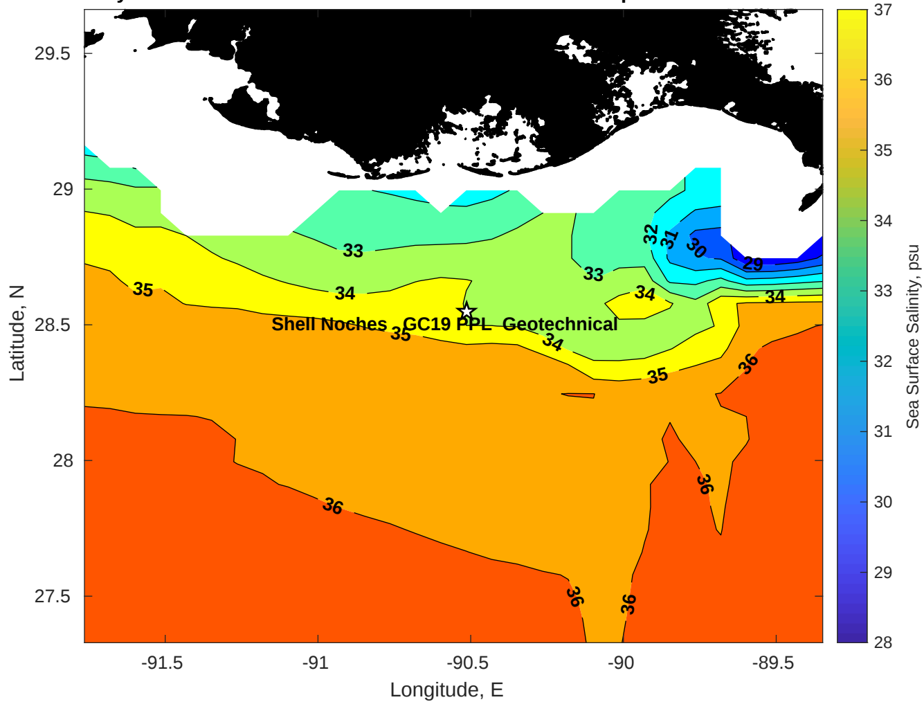
Surface Salinity for Shell Noches GC19 PPL Geotechnical at 25-Apr-2025 00:00:00
