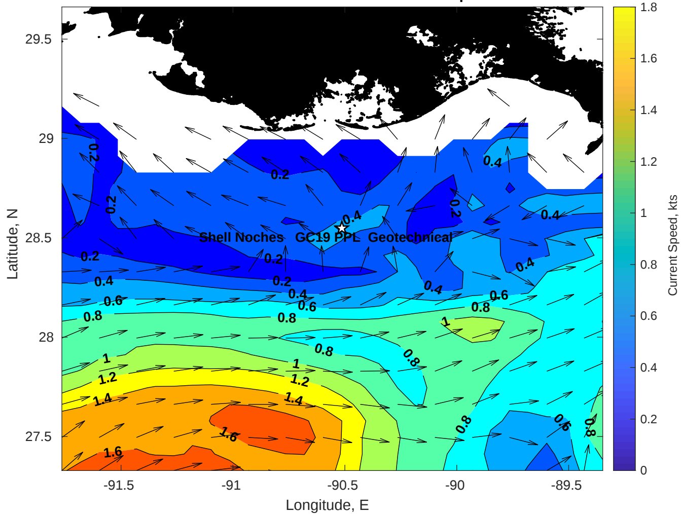
Surface Currents for Shell Noches GC19 PPL Geotechnical at 25-Apr-2025 00:00:00
