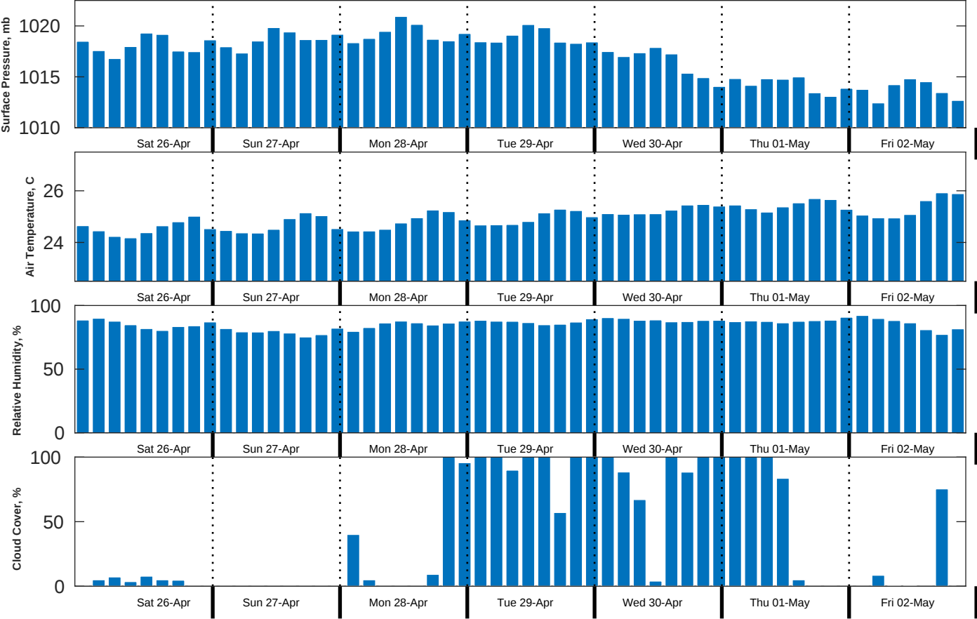
Met Forecast for Shell Noches GC19 PPL Geotechnical from 26-Apr-2025 00:00:00 to 03-May-2025 00:00:00
