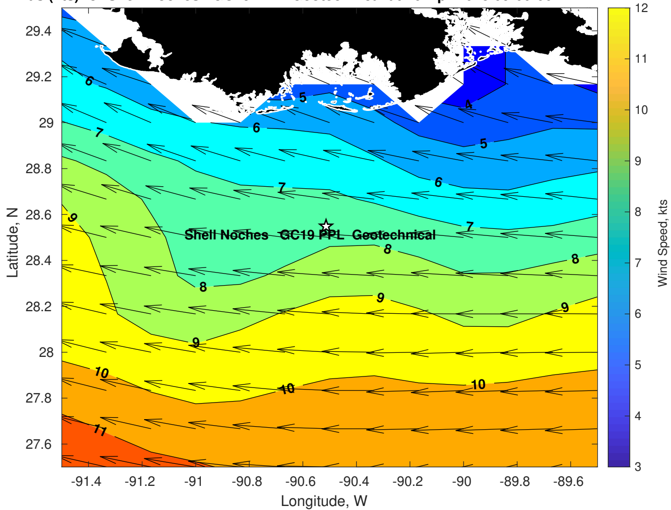
Winds (kts) for Shell Noches GC19 PPL Geotechnical at 26-Apr-2025 09:00:00
