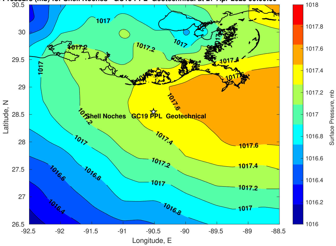
Surface Pressure (mb) for Shell Noches GC19 PPL Geotechnical at 27-Apr-2025 00:00:00
