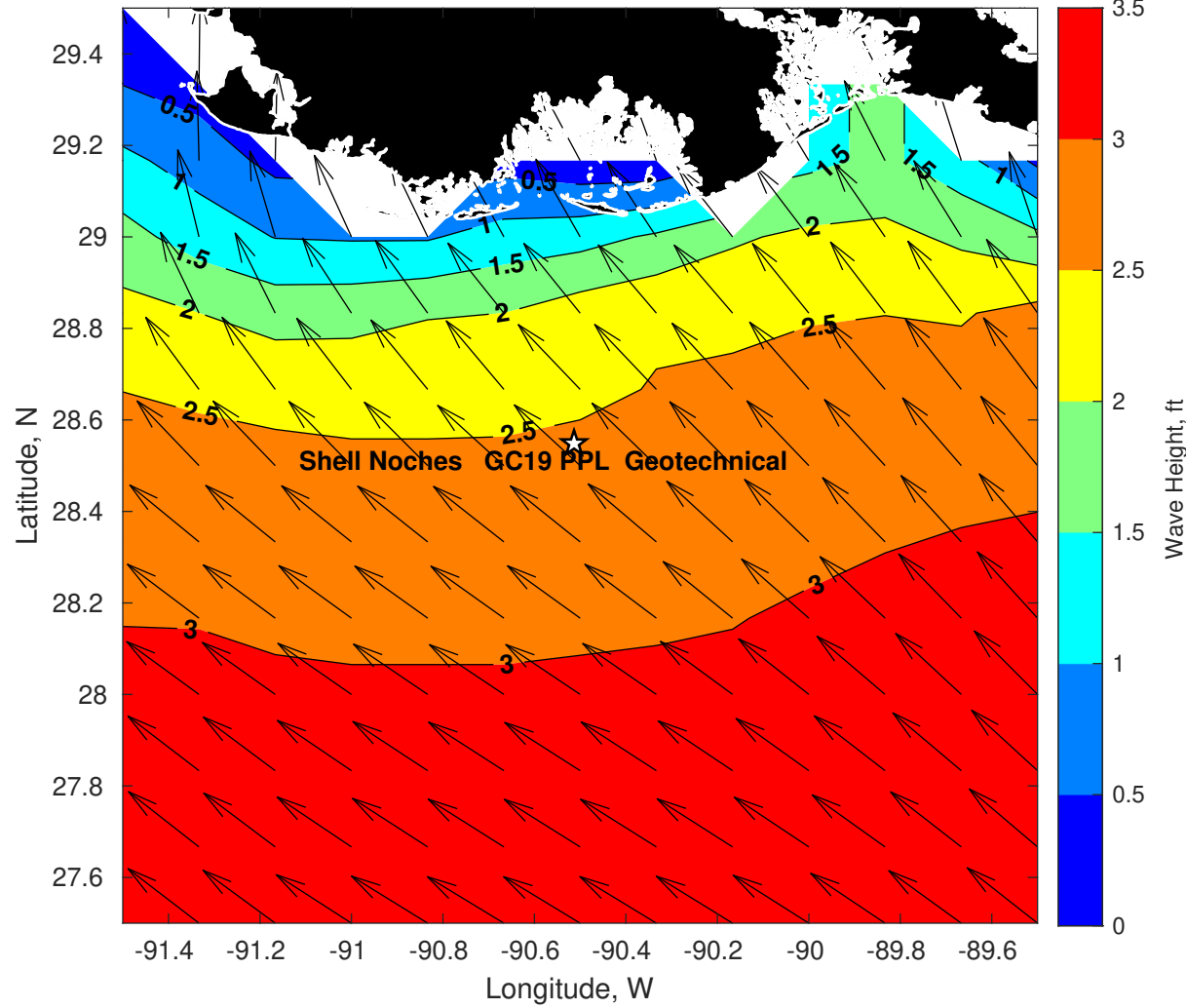
Wave Height (ft) for Shell Noches GC19 PPL Geotechnical at 26-Apr-2025 09:00:00
