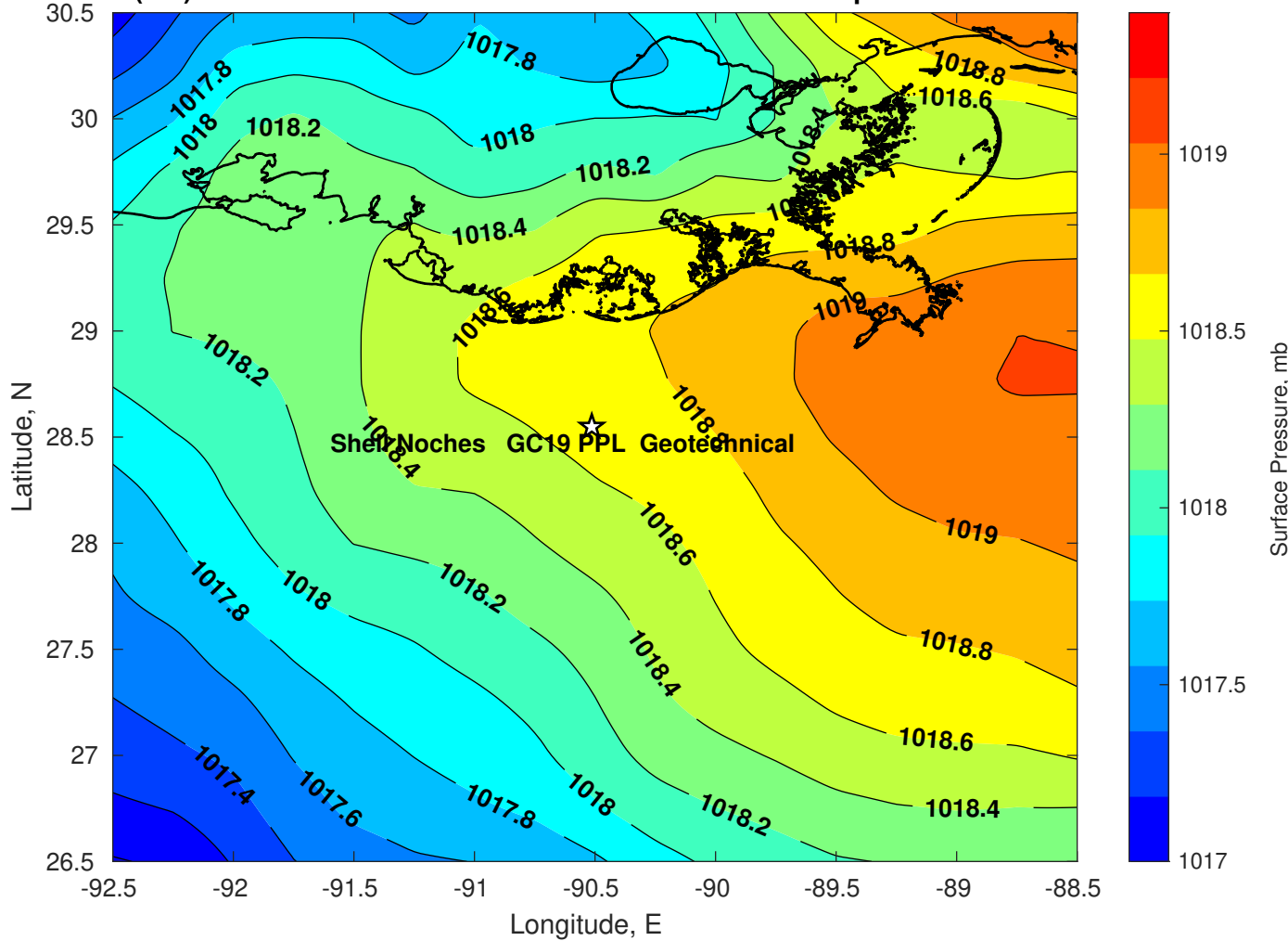
Surface Pressure (mb) for Shell Noches GC19 PPL Geotechnical at 28-Apr-2025 00:00:00
