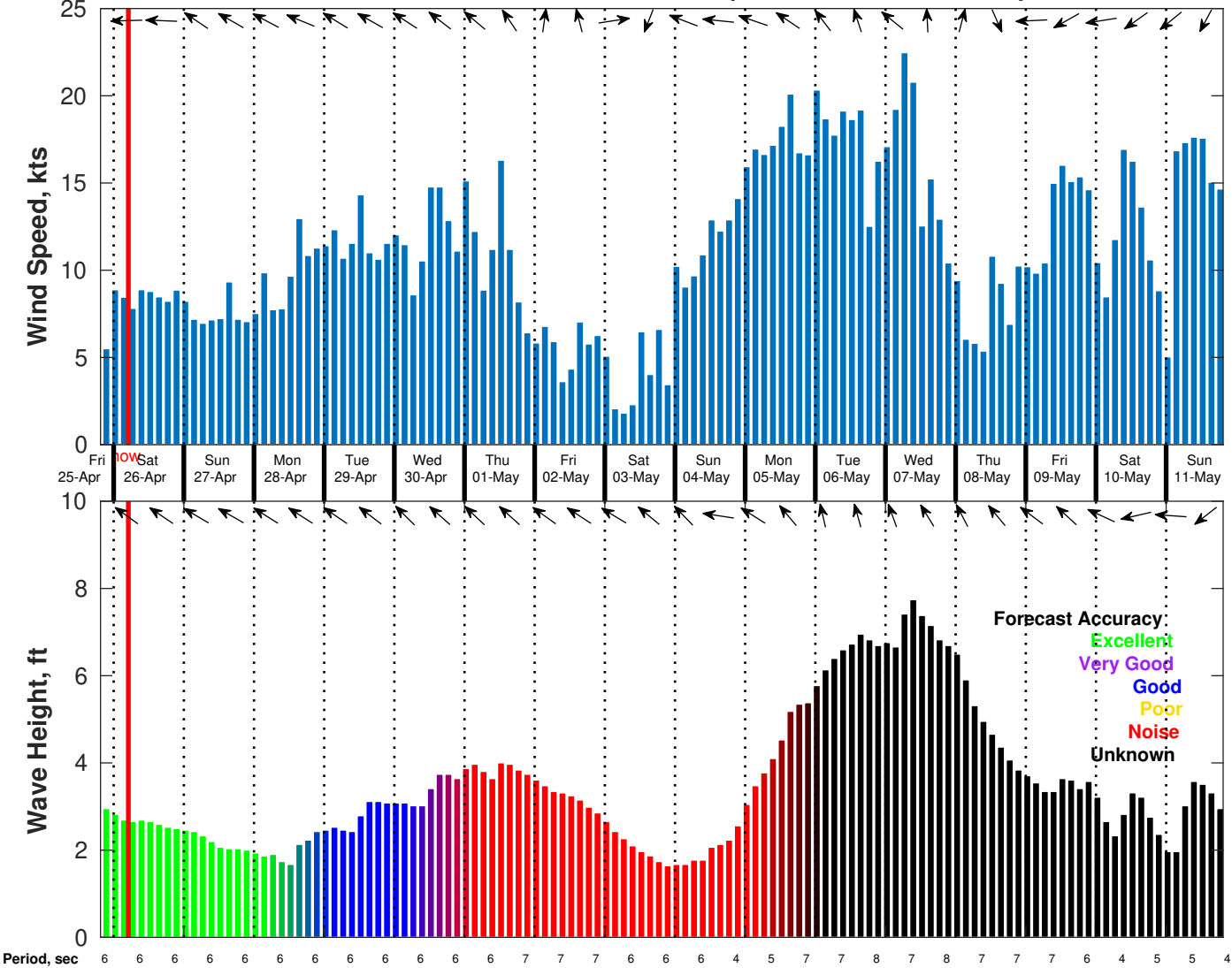
Wind & Wave Forecast for Shell Noches GC19 PPL Geotechnical from 25-Apr-2025 20:00:00 to 11-May-2025 20:00:00
