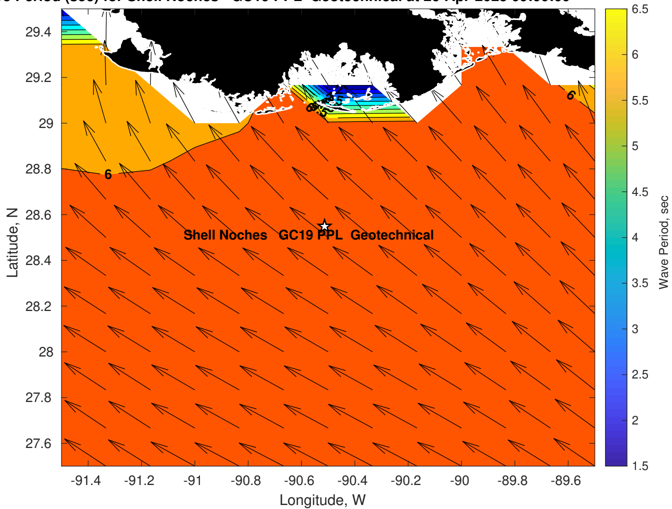
Wave Period (sec) for Shell Noches GC19 PPL Geotechnical at 26-Apr-2025 09:00:00
