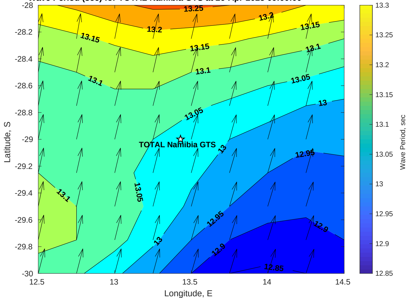
Wave Period (sec) for TOTAL Namibia GTS at 26-Apr-2025 09:00:00
