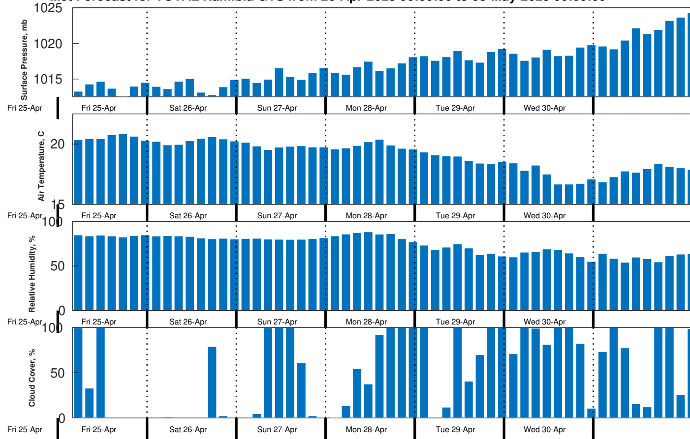
Met Forecast for TOTAL Namibia GTS from 26-Apr-2025 00:00:00 to 03-May-2025 00:00:00
