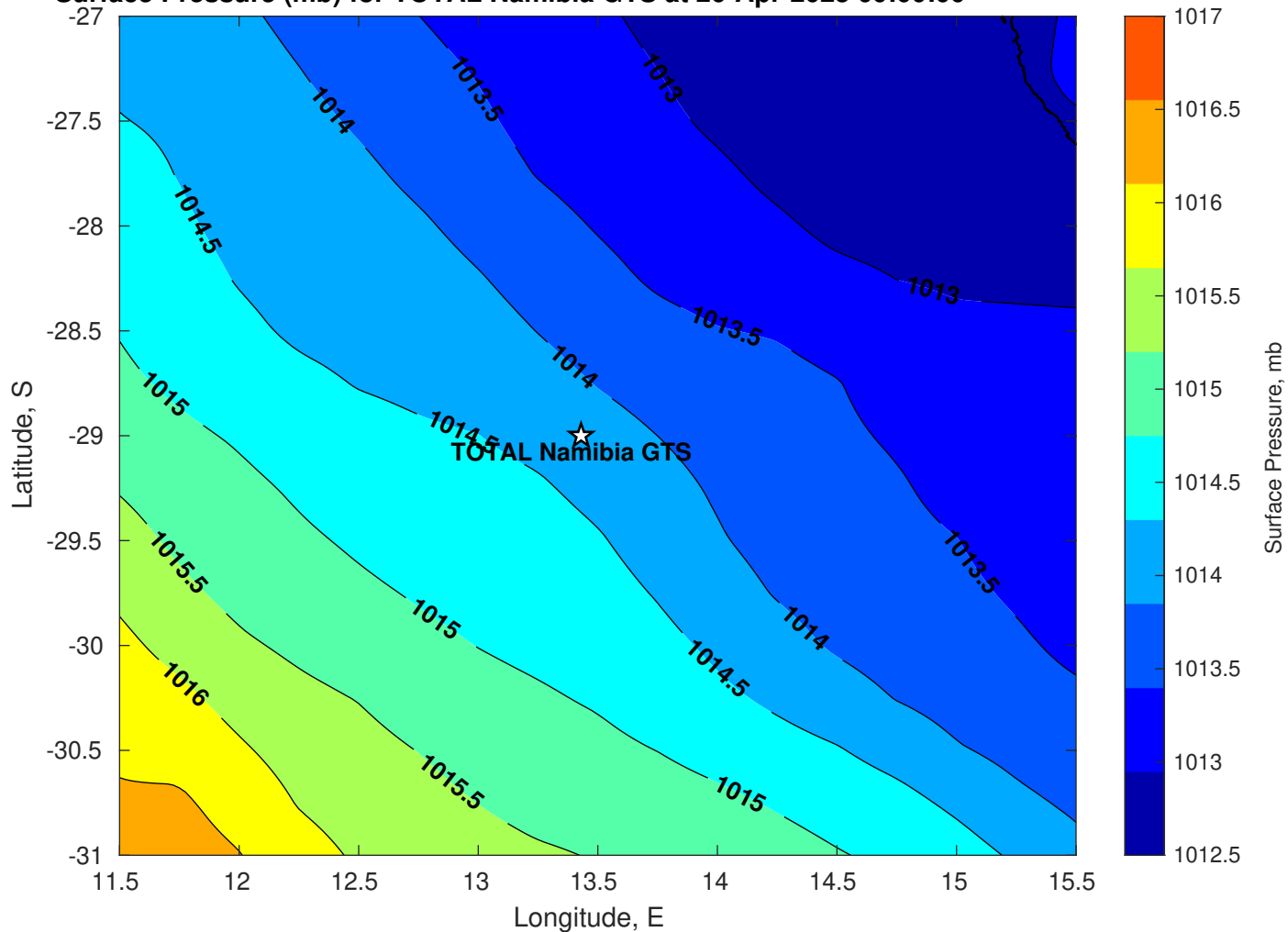
Surface Pressure (mb) for TOTAL Namibia GTS at 26-Apr-2025 00:00:00
