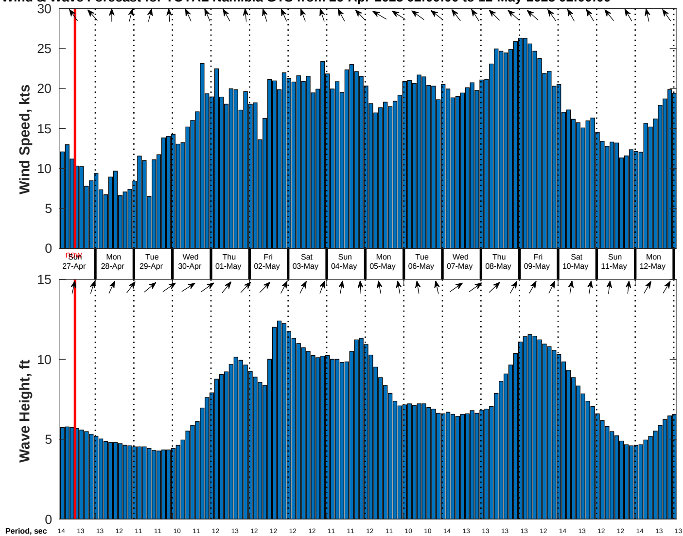
Wind & Wave Forecast for TOTAL Namibia GTS from 26-Apr-2025 02:00:00 to 12-May-2025 02:00:00
