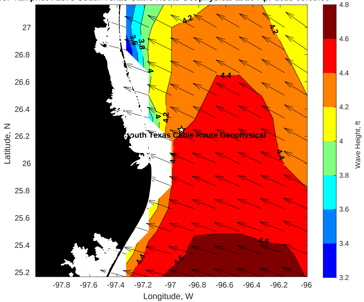
Wave Height (ft) for Tampnet P2378 South Texas Cable Route Geophysical at 26-Apr-2025 09:00:00
