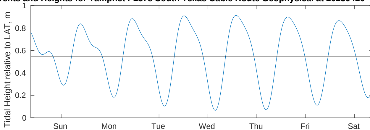
Tidal Currents and Heights for Tampnet P2378 South Texas Cable Route Geophysical at 20250426
