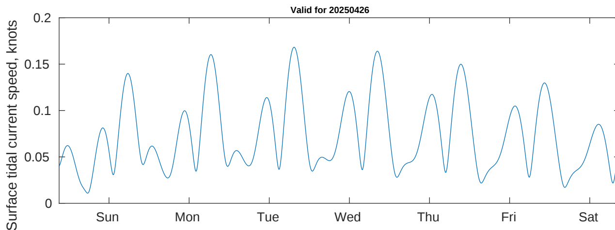
Tidal Currents and Heights for Tampnet P2378 South Texas Cable Route Geophysical at 20250426
