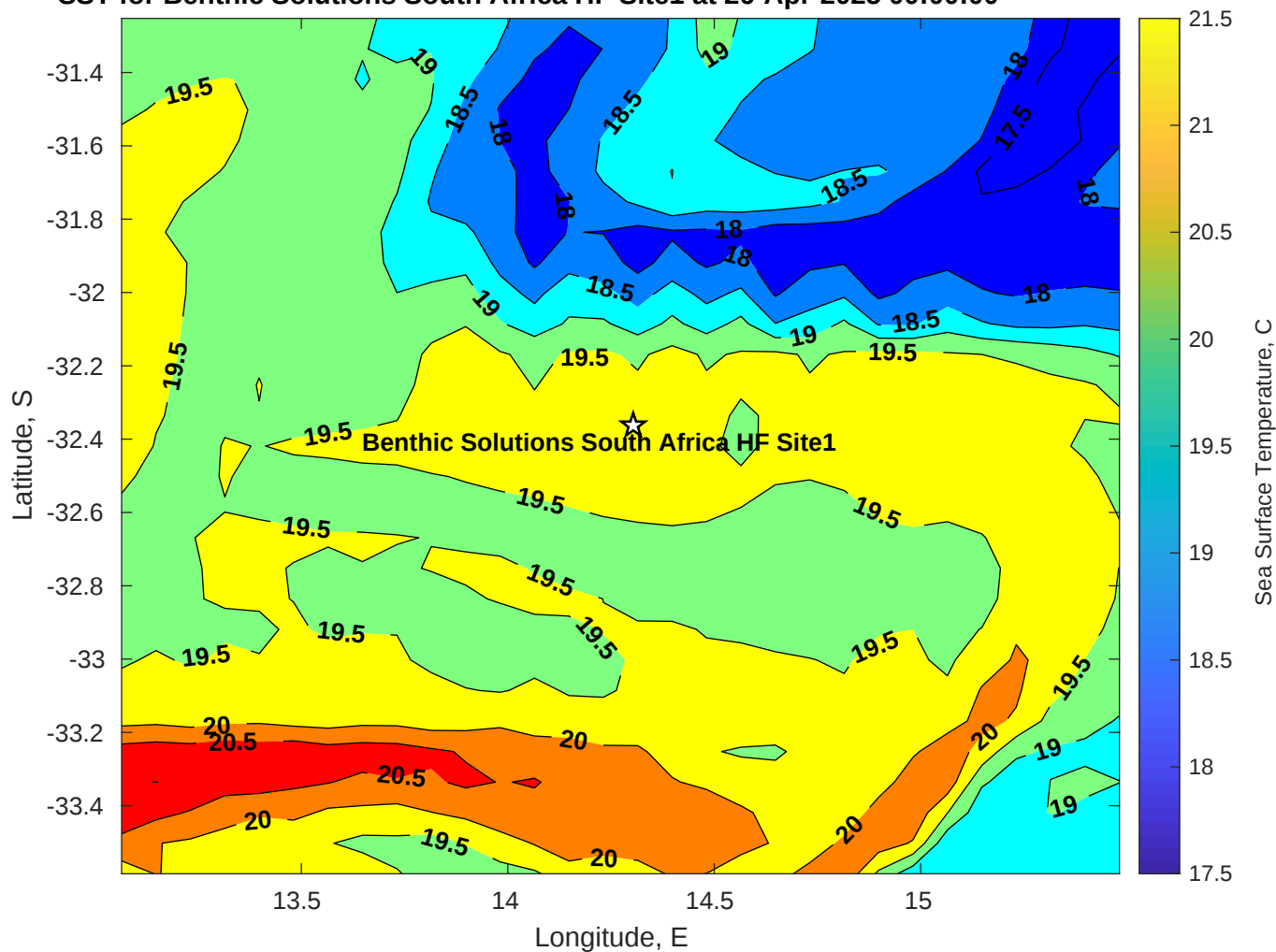
SST for Benthic Solutions South Africa HF Site1 at 26-Apr-2025 00:00:00
