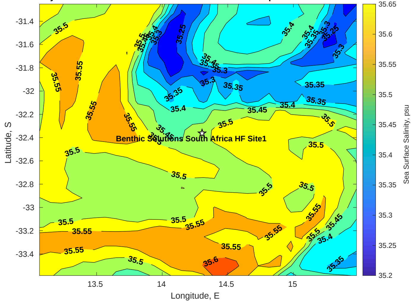
Surface Salinity for Benthic Solutions South Africa HF Site1 at 26-Apr-2025 00:00:00
