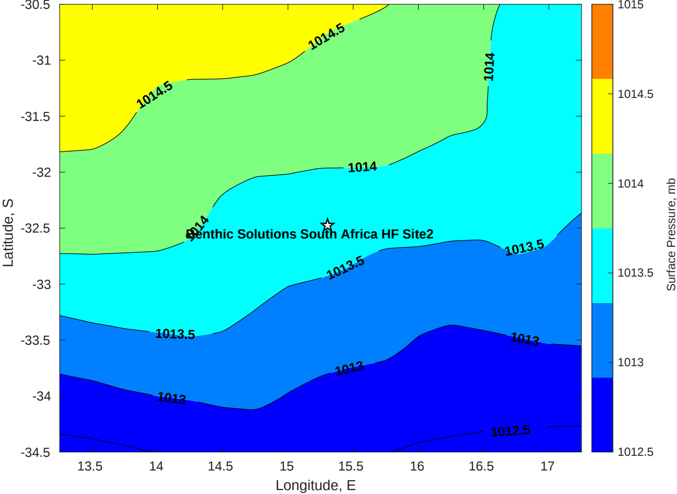
Surface Pressure (mb) for Benthic Solutions South Africa HF Site2 at 28-Apr-2025 00:00:00
