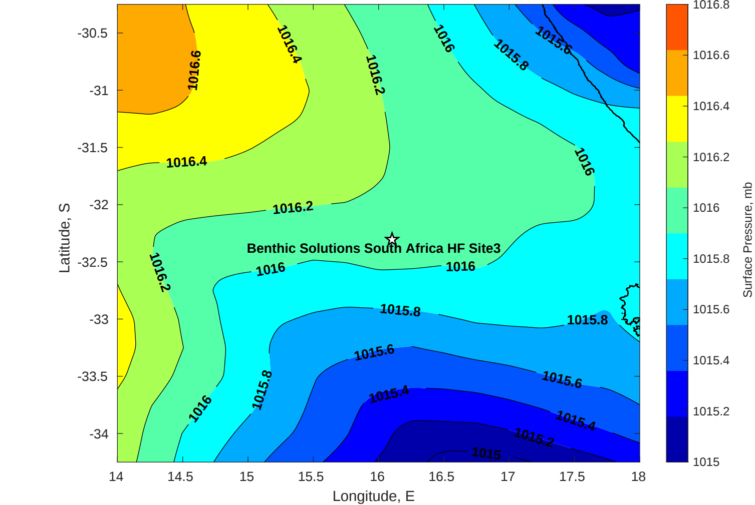
Surface Pressure (mb) for Benthic Solutions South Africa HF Site3 at 29-Apr-2025 00:00:00
