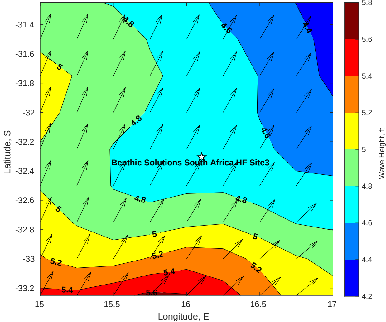
Wave Height (ft) for Benthic Solutions South Africa HF Site3 at 27-Apr-2025 09:00:00
