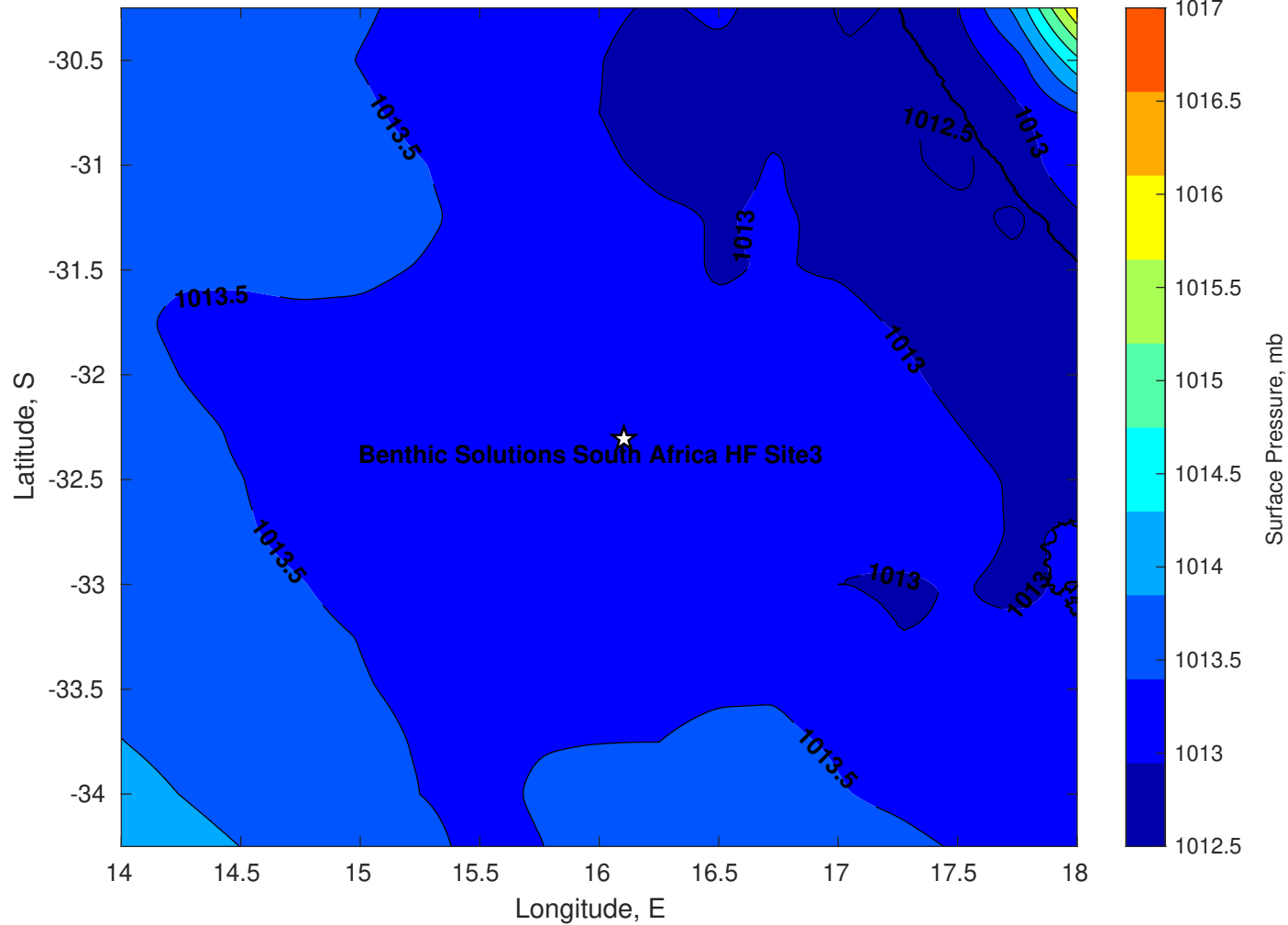
Surface Pressure (mb) for Benthic Solutions South Africa HF Site3 at 27-Apr-2025 00:00:00
