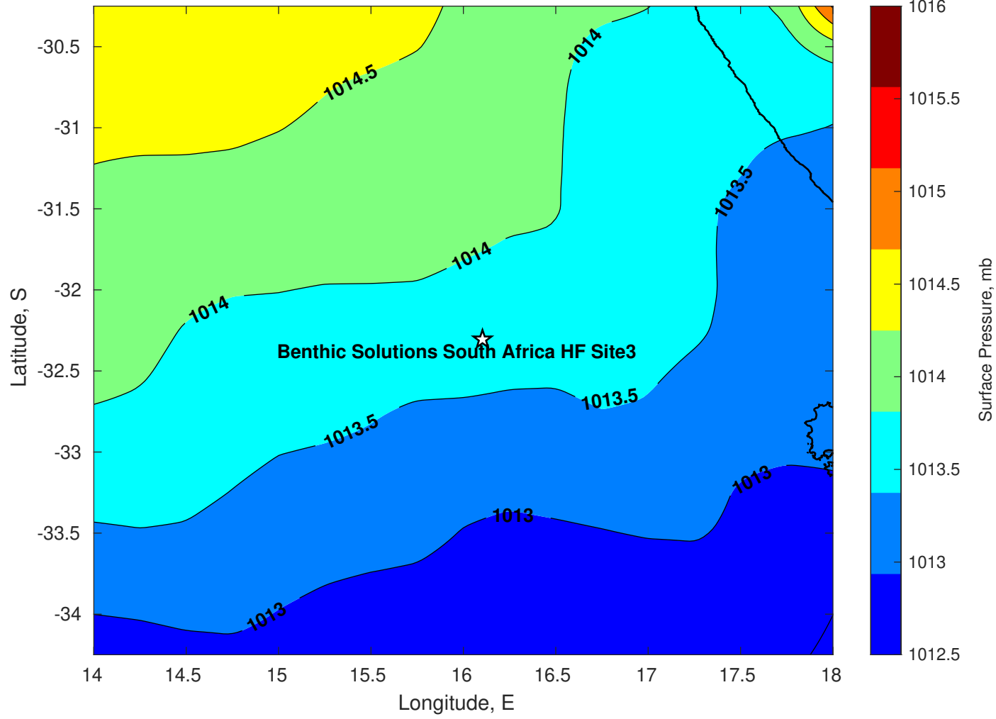
Surface Pressure (mb) for Benthic Solutions South Africa HF Site3 at 28-Apr-2025 00:00:00
