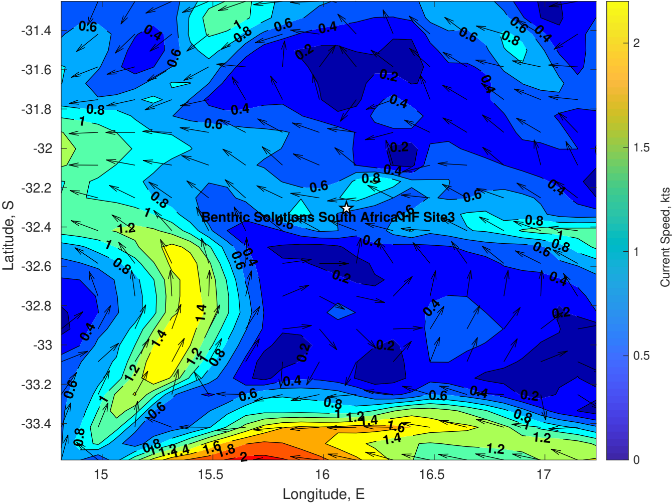
Surface Currents for Benthic Solutions South Africa HF Site3 at 26-Apr-2025 00:00:00
