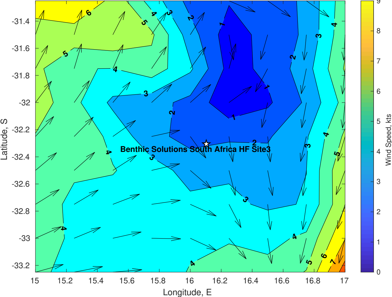
Winds (kts) for Benthic Solutions South Africa HF Site3 at 27-Apr-2025 09:00:00
