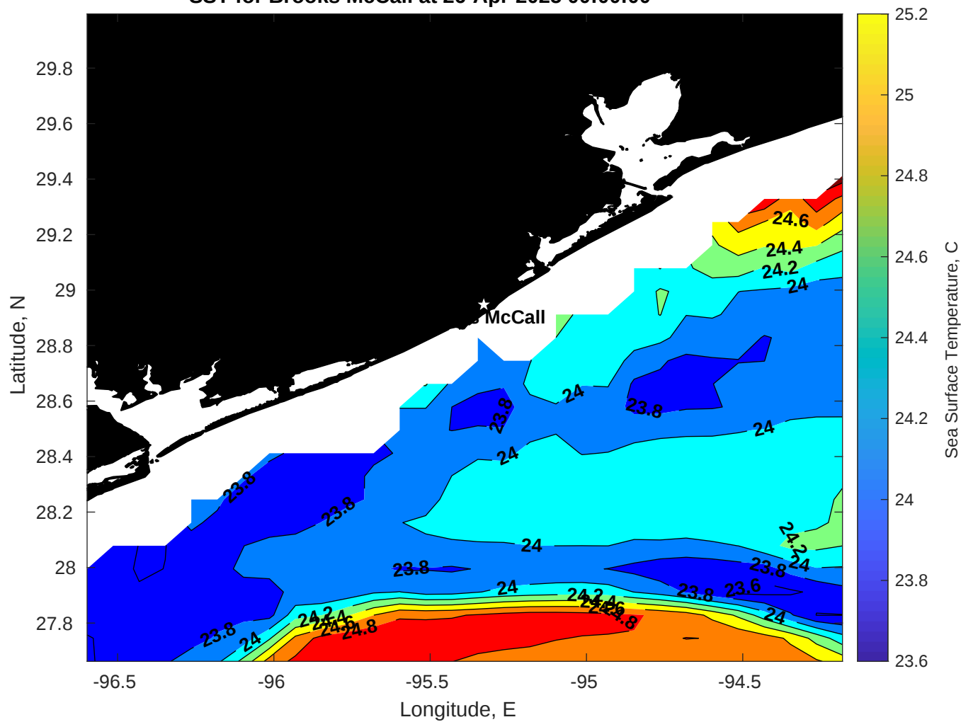
SST for Brooks McCall at 26-Apr-2025 00:00:00
