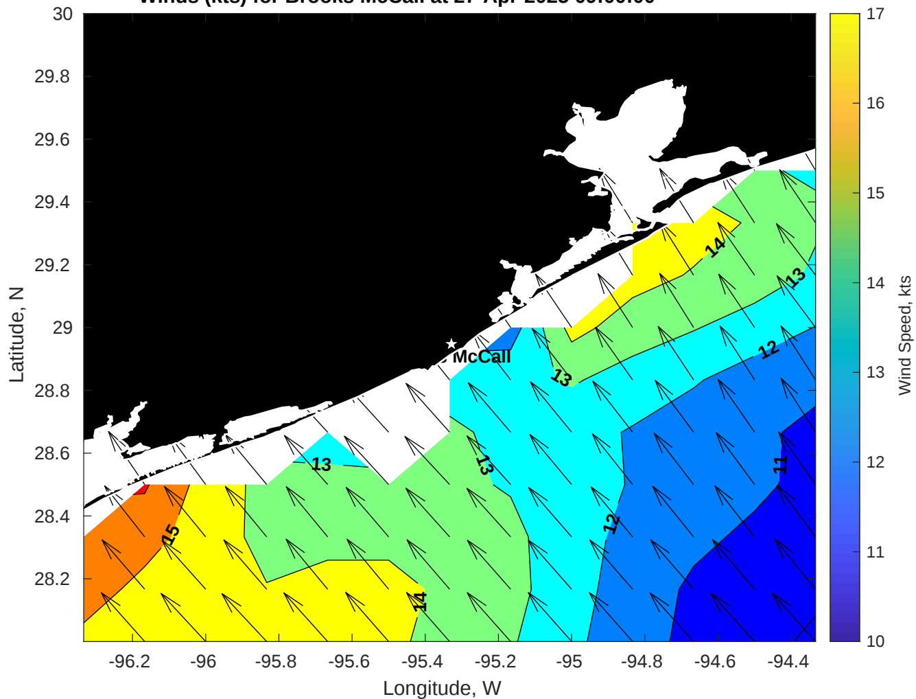
Winds (kts) for Brooks McCall at 27-Apr-2025 09:00:00
