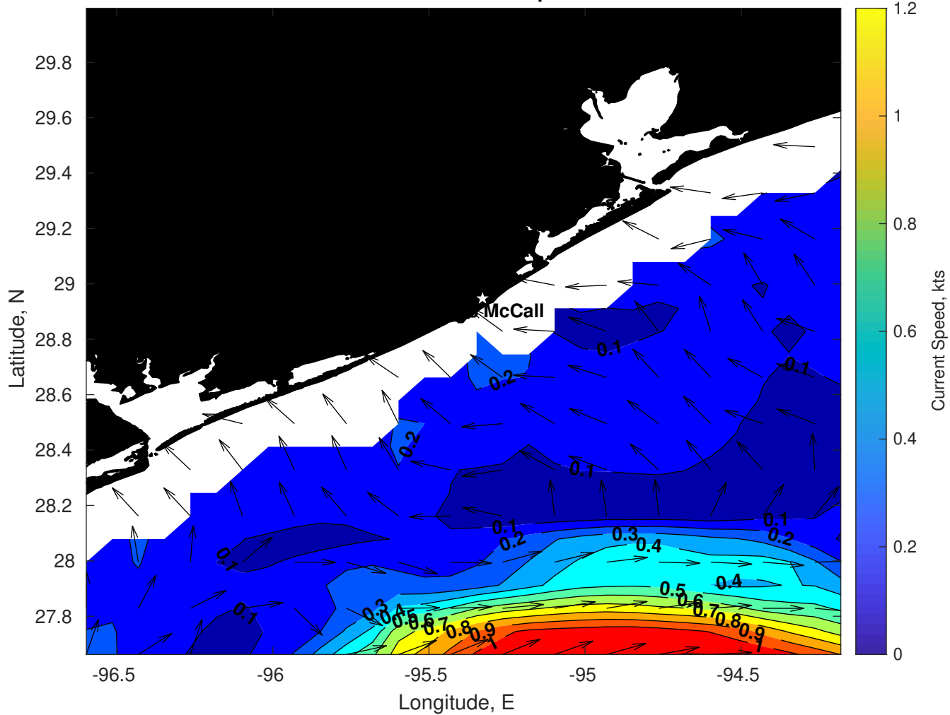
Surface Currents for Brooks McCall at 26-Apr-2025 00:00:00
