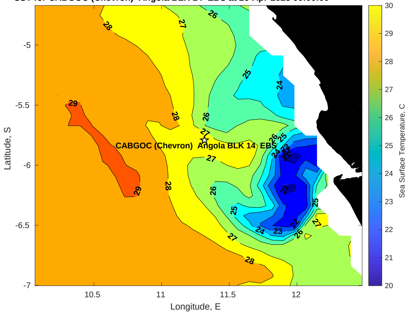
SST for CABGOC (Chevron) Angola BLK 14 EBS at 26-Apr-2025 00:00:00
