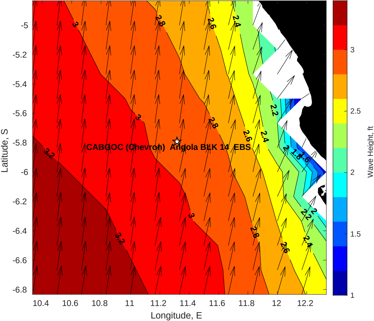
Wave Height (ft) for CABGOC (Chevron) Angola BLK 14 EBS at 27-Apr-2025 09:00:00
