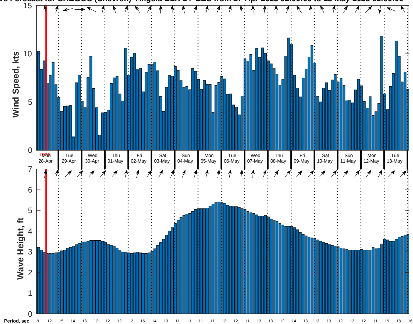
Wind & Wave Forecast for CABGOC (Chevron) Angola BLK 14 EBS from 27-Apr-2025 02:00:00 to 13-May-2025 02:00:00
